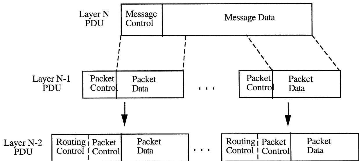
Figure 2 The data units at each of the three layers.
