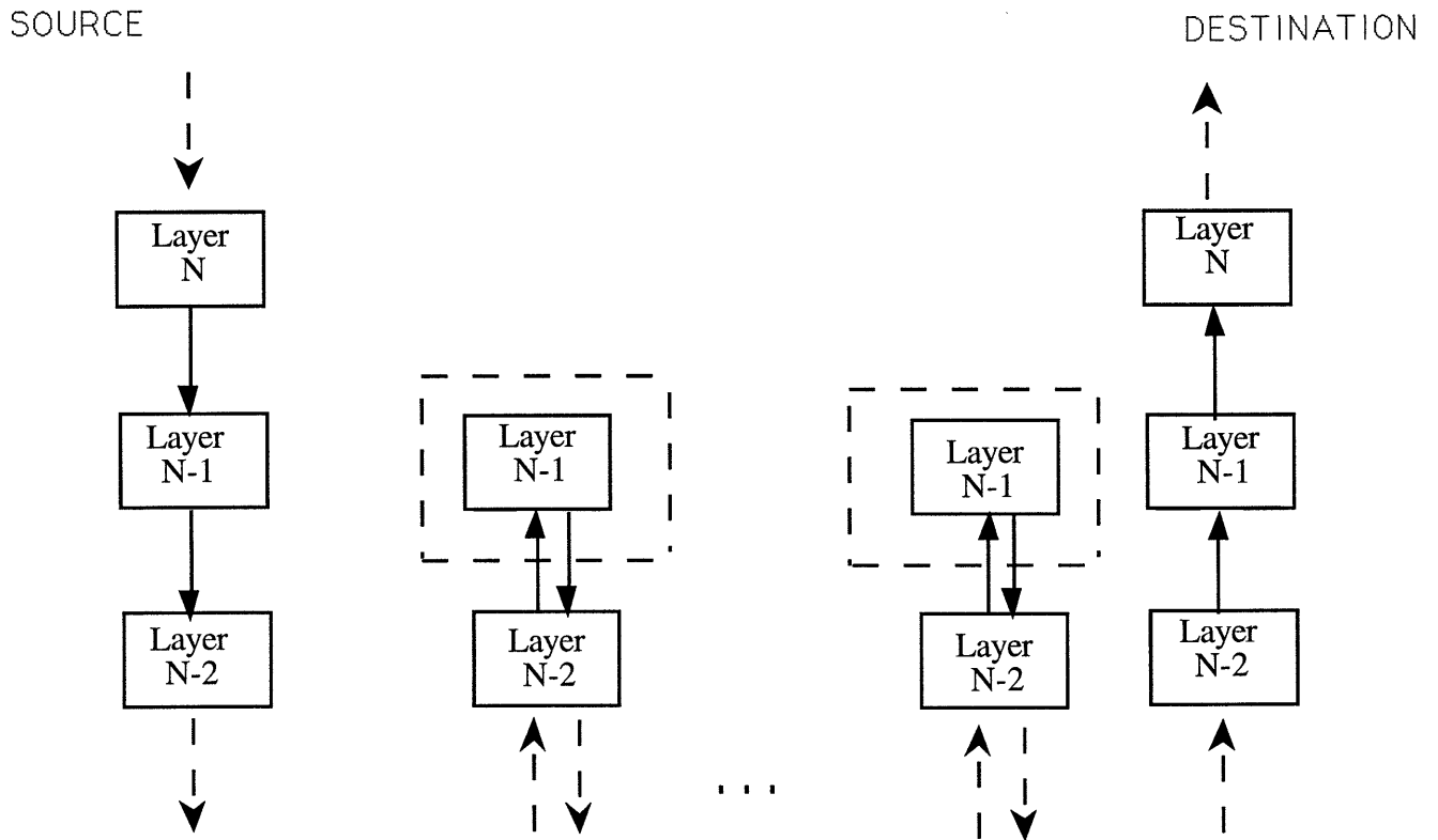
Figure 1 The layers of interest along the data path. Layer N-1 is shown in dotted lines at the intermediate nodes since it possibly may fragment the packets further at these nodes, but it does not put the packets together to form a message until the destination.
