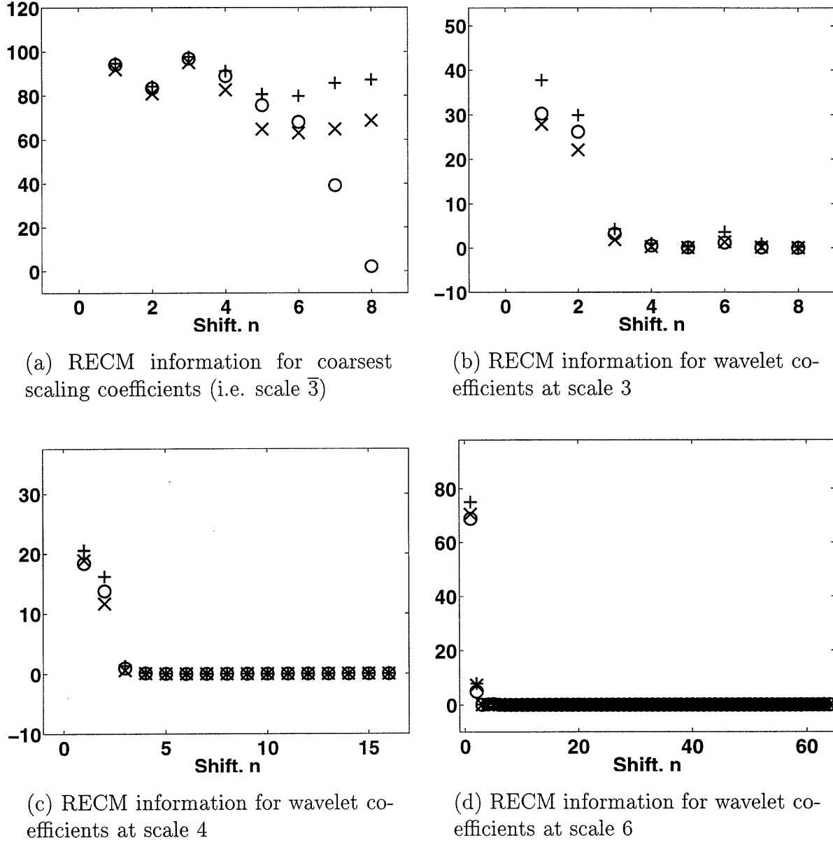
Figure 6: Diagonal elements of relative error covariances for three radial profiling experiments. In all cases, the symbol “+” corresponds to \Pi(D_{HI,MID}) , “o” to \Pi(D_{HI}) and “x” to \Pi(D_{MID}) . From (a) we see a significant level of sensor fusion taking place with respect to the estimates of the coarsest scale scaling coefficients far from the origin x = 0 . From (b)–(d), we conclude that accurate reconstruction of the detail components of g is limited to shifts close to x = 0 .
