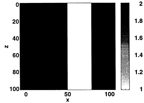
(d) The finest scale of to which x -oriented detail can be reconstructed at \tau = 0.5 given high, middle, and low frequency data.
