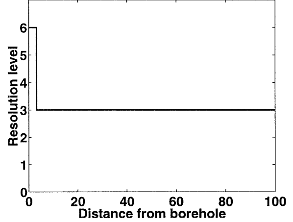
(b) The optimal scale of reconstruction as a function of position at scale M_g = 7 for a threshold value of \tau = 0.50 .
