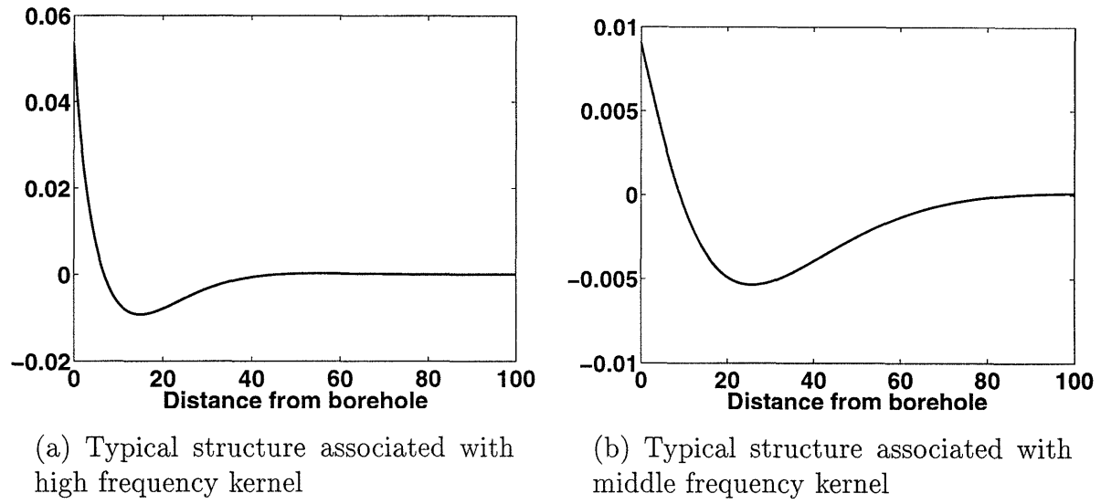
Figure 4: Typical structure of kernel functions used in the reconstruction of g for the radial profiling example.
