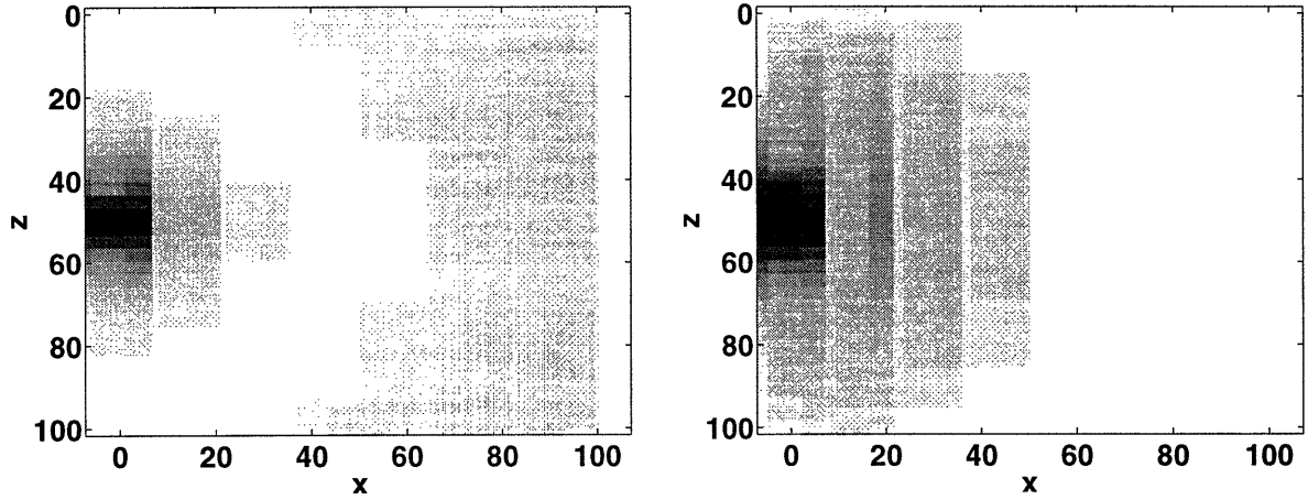
(a) Structure of typical high frequency kernel
