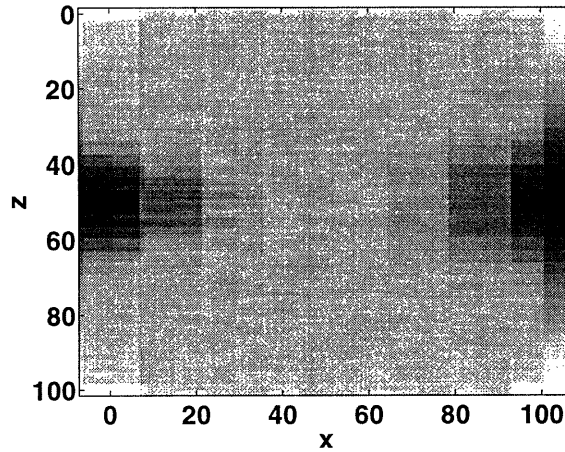
(c) Structure of typical low frequency kernel
