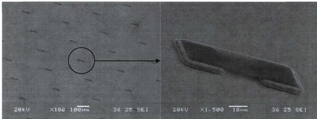
Figure 10. SiO 2 etched away to create air gap under polymer material
