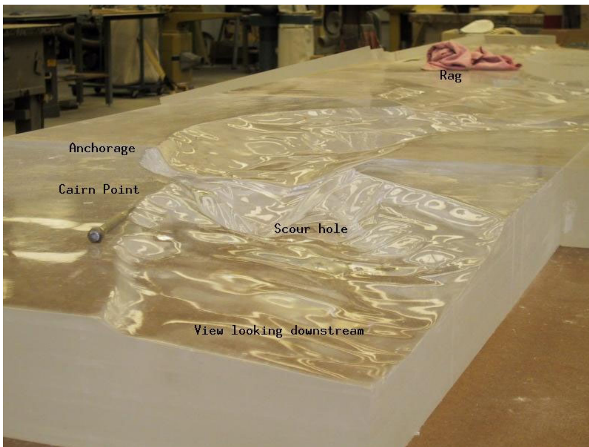
Figure 6. Portion of 3-D Cook Inlet model looking downstream
