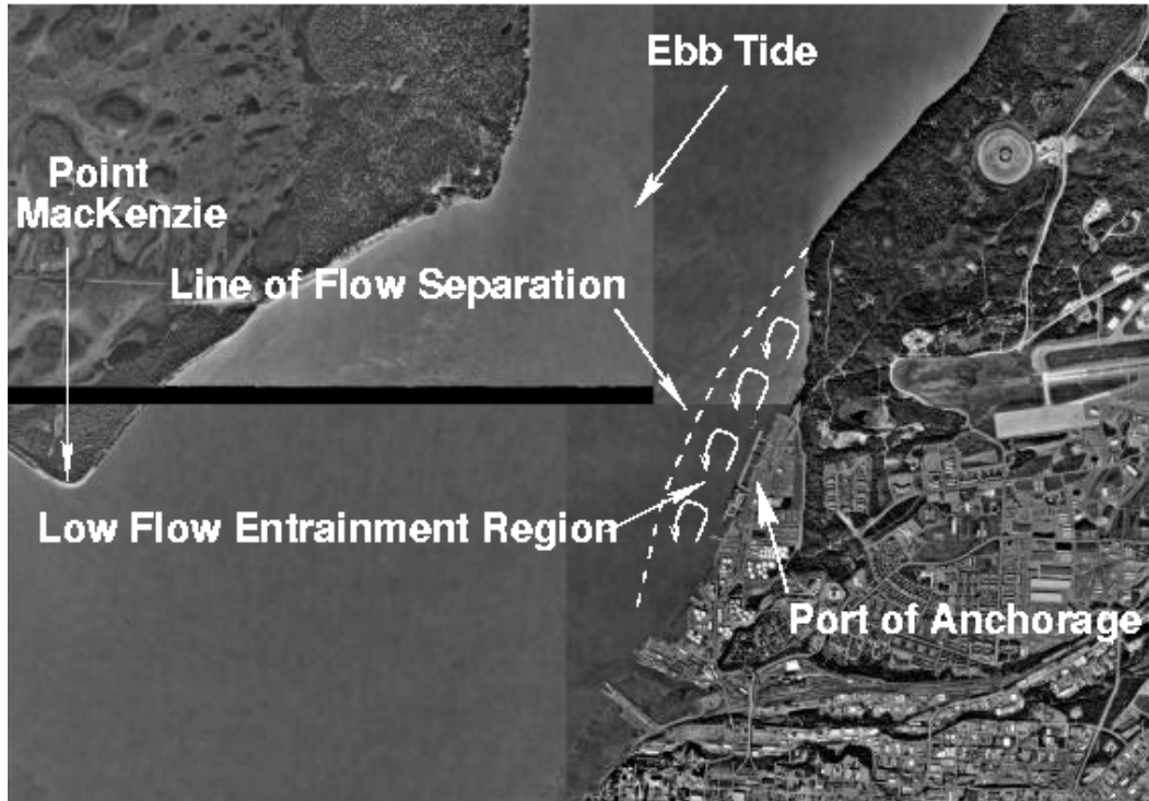
Figure 3. Flow separation off Cairn Point during ebb flow (Cook Inlet, AK)
