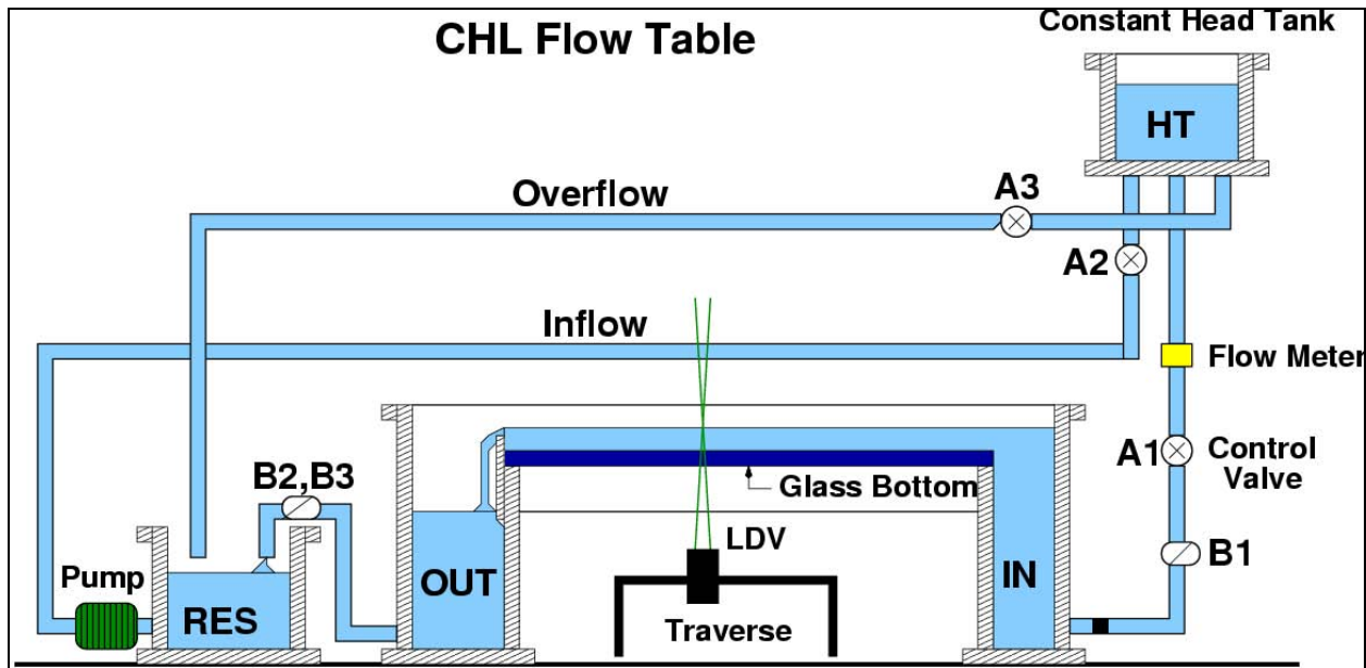
Figure 1. Schematic side-view showing flow table components
