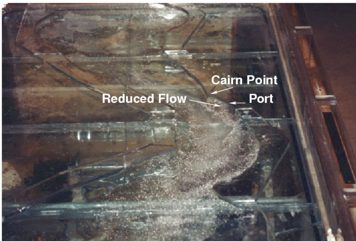
Figure 7. Surface flow tracer showing reduced flow at Port of Anchorage during ebb tide
