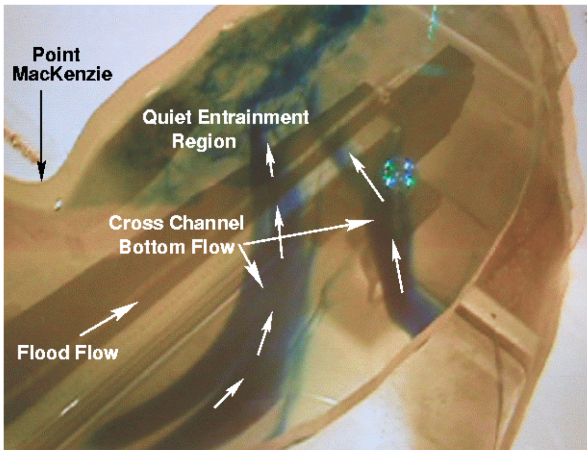
Figure 5. Cross-channel bottom flow at Cook Inlet, AK
