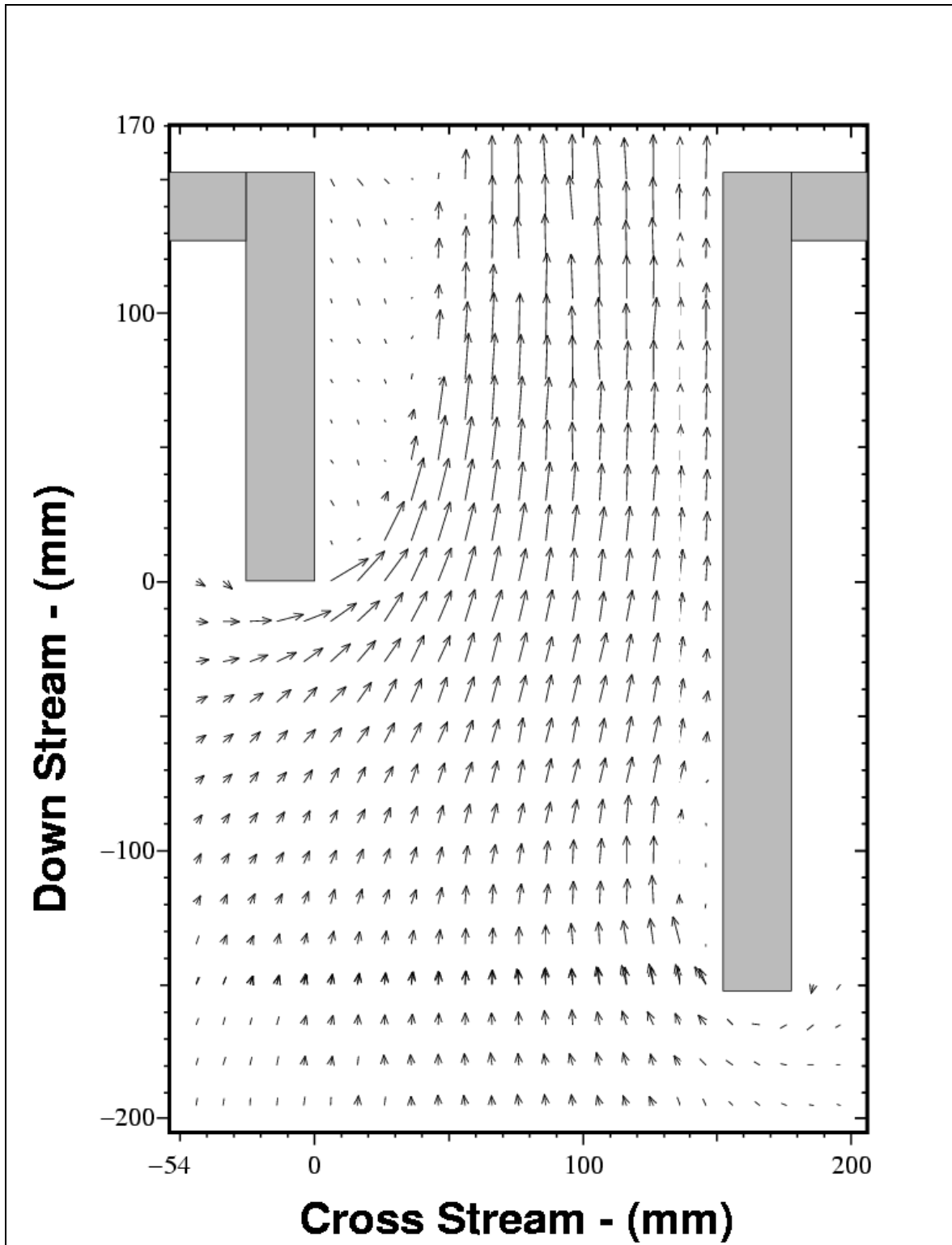
Figure 2. Velocity field at unequal length jetties
