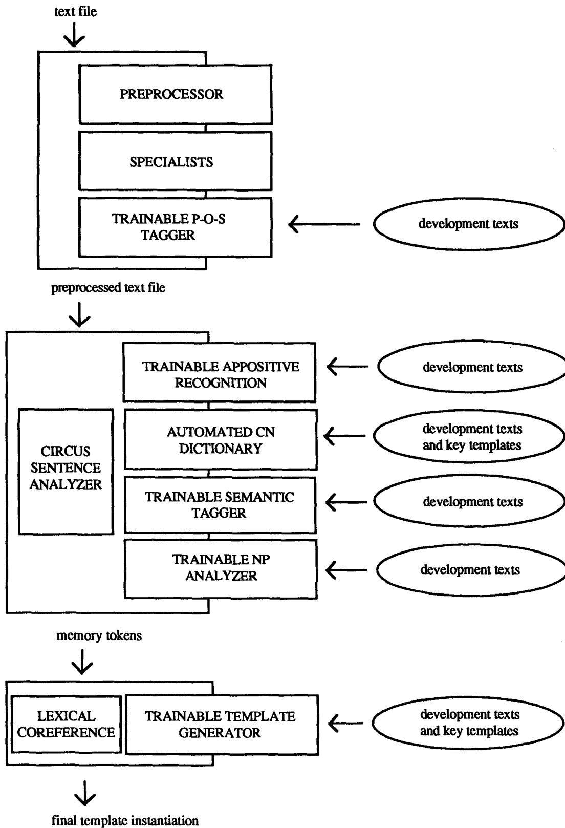
Figure 1: System Architecture
