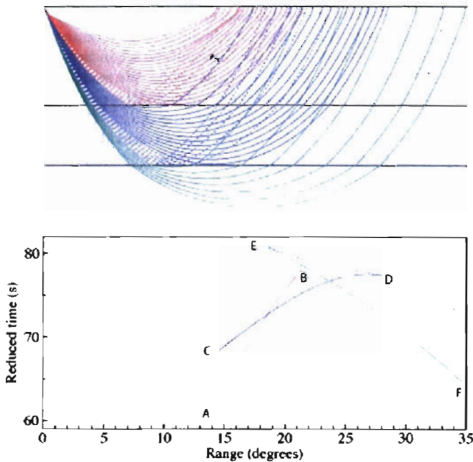
Figure 1. Discontinuities in the mantle transition zone at 410- and 660-km depths cause a pair of triplications in P- and S-wave arrivals between ~15 and 30 degrees. The ray paths (top) are color-coded and correspond to the different branches in the travel-time curve plotted below (reduced at 10 s/degree). The AB branch consists of direct waves that bottom above the 410-km discontinuity (red solid). The BC branch reflects at 410 km (red dashed). The CD and DE branches bottom above and reflect off the 660-km discontinuity (blue solid and dashed). The EF branch bottoms in the lower mantle. This figure is adopted from Shearer (2000).
