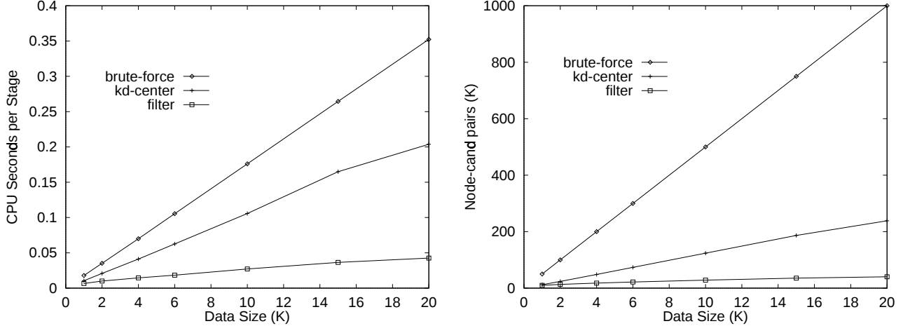
Figure 5: Running time and node-candidate pairs versus data size, for k = 50 and \sigma = 0.10 .
