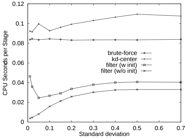
Figure 4: Average CPU time and node-candidate pairs per stage versus cluster standard deviation, for n = 10,000 and k = 20 .
