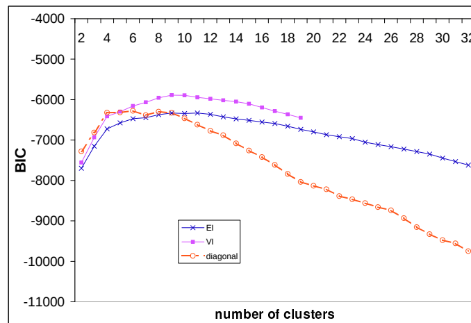
Figure 10: Average BIC values for the log transformed ovary data.
