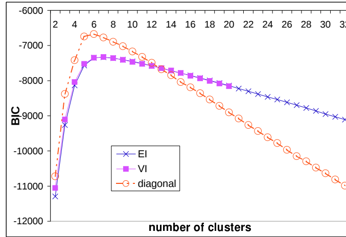
Figure 6: Average BIC values for the synthetic cyclic data sets.
