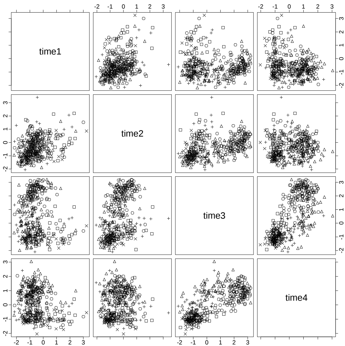
Figure 18: Pairs plot of the standardized yeast cell cycle data with the 5-phase criterion.
