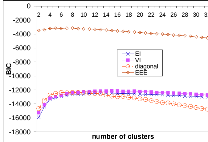
Figure 16: Average BIC values for the standardized yeast cell cycle data with the 5-phase criterion.
