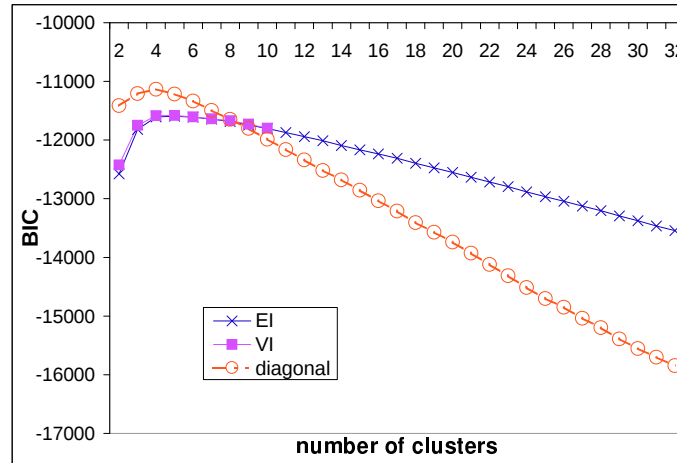
Figure 4: Average BIC values for the synthetic randomly resampled ovary data.
