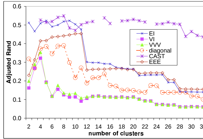
Figure 19: Adjusted Rand indices for the standardized yeast cell cycle data with the MIPS criterion.
