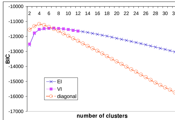
Figure 2: Average BIC values for synthetic data based on the ovary data: Mixture of 4 multivariate normal distributions
