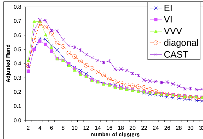
Figure 1: Average adjusted Rand indices for the synthetic data based on the ovary gene expression data: Mixture of 4 multivariate normal distributions
