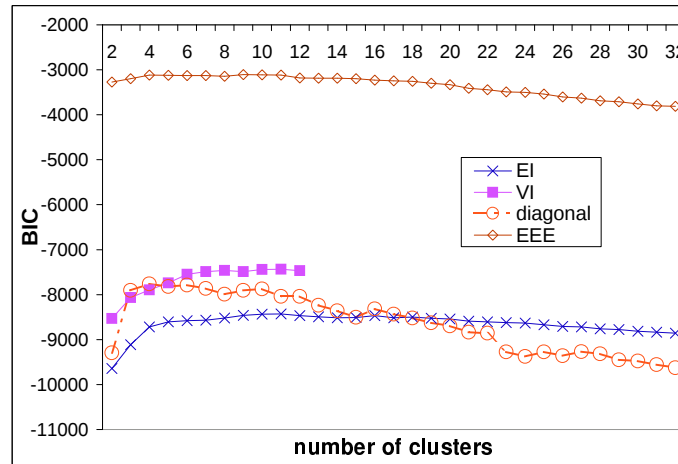
Figure 20: BIC values for the standardized yeast cell cycle data with the MIPS criterion.
