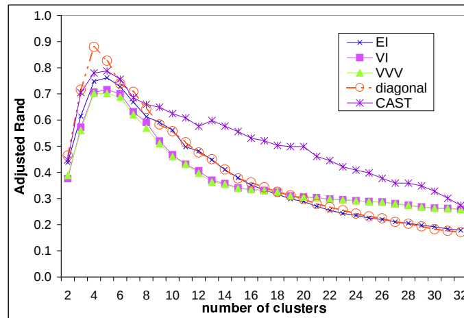
Figure 3: Average adjusted Rand indices for the synthetic randomly resampled ovary data sets.
