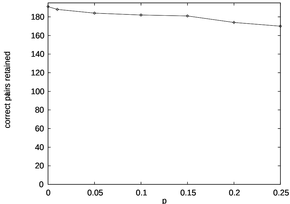
Figure 3: The length filter eliminates few correct pairs.
