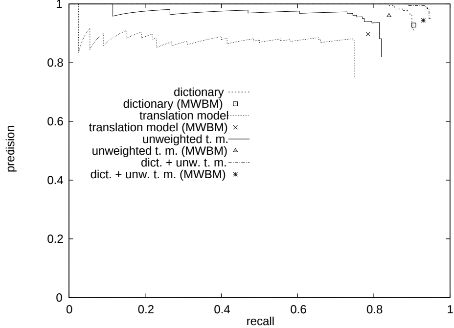
Figure 7: Precision and recall of four t functions through the competitive linking process and under maximum weighted bipartite matching.
