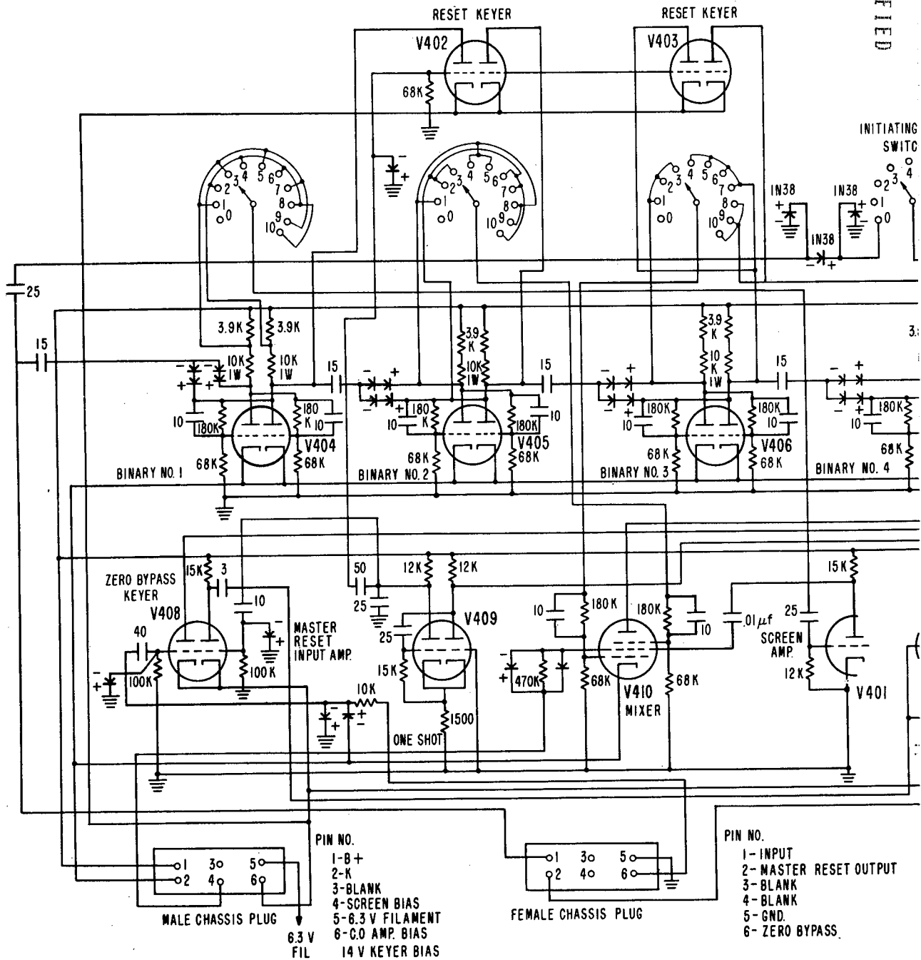
Figure 8 - Schematic diagram of thousands decade
