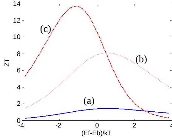
Fig. 7. Thermoelectric figure of merit versus reduced Fermi energy for three models.
