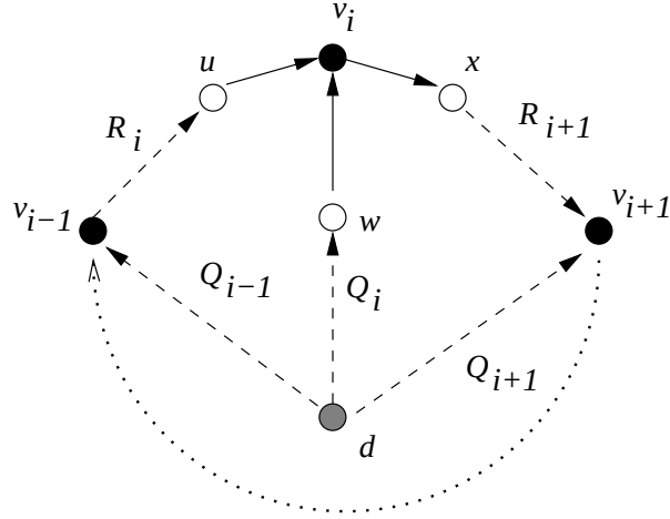
Figure 2: Dispute wheel.
