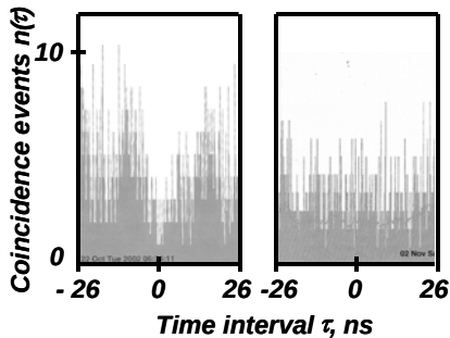
Fig. 1. Left histogram exhibits a dip at \tau = 0 indicating photon antibunching in the fluorescence of the single molecule; no antibunching is observed in the fluorescence from the assembly of several molecules (right histogram).
