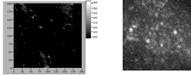
Figure 11. Single-quantum dot fluorescence imaging in 1-D photonoc bandgap cholesteric liquid crystal host by 40 \mu\text{m} x 40 \mu\text{m} raster scan (left) and EM-CCD-camera (right).
