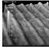
Fig. 5. Left: Perspective view of the AFM-topographical image of a planar-aligned chiral liquid crystal oligomer ( 1.12\mu\text{m} \times 1.12\mu\text{m} scan); Center: Selective reflection curves of left-handed circularly polarized light from 1-D photonic band gap chiral liquid crystal oligomers; Right: Near-field optical image of 2-D self-assembly of a planar-aligned chiral liquid crystal oligomer ( 5\mu\text{m} \times 5\mu\text{m} scan)
