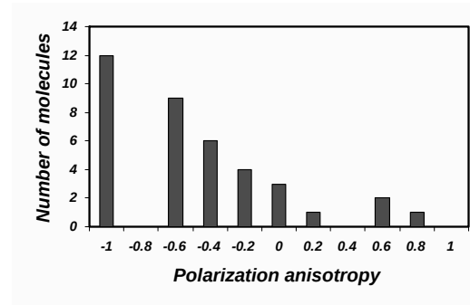
Fig. 3. The histogram of polarization anisotropy of 38 molecules of DiIC 18 (3) dye in planar aligned glassy nematic liquid crystal host (See details in Section 8).
