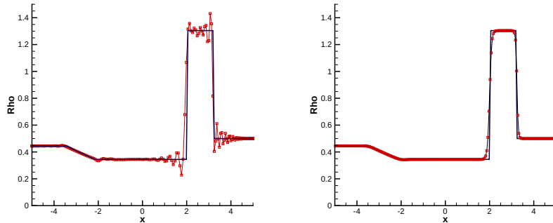
Fig. 1. The density of the Lax problem as computed by (Left) the Chebyshev collocation solution with the Gibbs oscillations and (Right) the fifth-order characteristic-wise WENO finite difference scheme. The exact solution is represented by the solid line.
