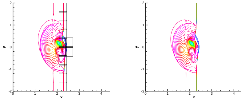
Fig. 11. Density contour of the Shock-Vortex interaction with Mach number M_s = 3 and vortex strength \Gamma = 0.25 at t = 0.6 . Hybrid (Left); Classical WENO (Right). WENO subdomains are denoted by bounding boxes.
