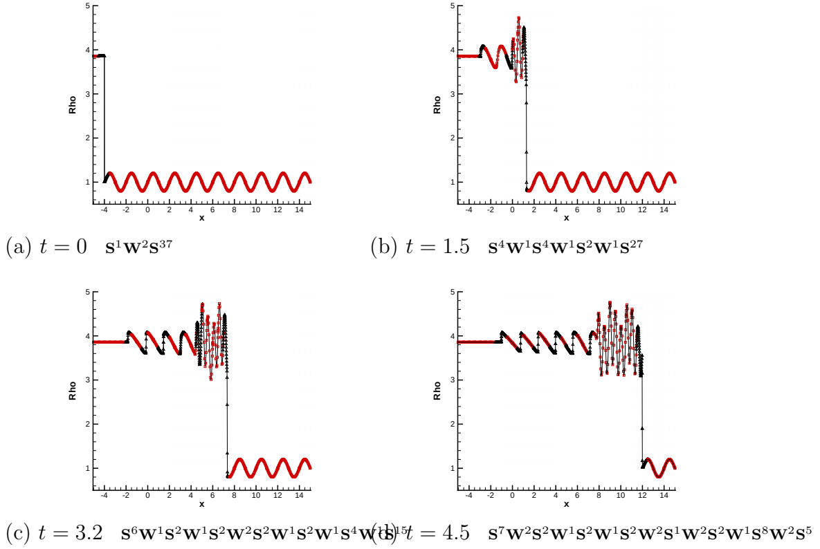
Fig. 10. The density profile of the Mach 3 Shock-Entropy wave interaction at times (a) t = 0 , (b) t = 1.5 , (c) t = 3.2 and (d) t = 4.5 with 40 subdomains, as indicated by the vertical lines. N_s = 16 , N_w = 50 and \epsilon_{MR} = 5 \times 10^{-3} . Spectral ( \square ); WENO ( \triangle ); The solid line is the solution computed with the fifth order WENO scheme with 2000 grid points.
