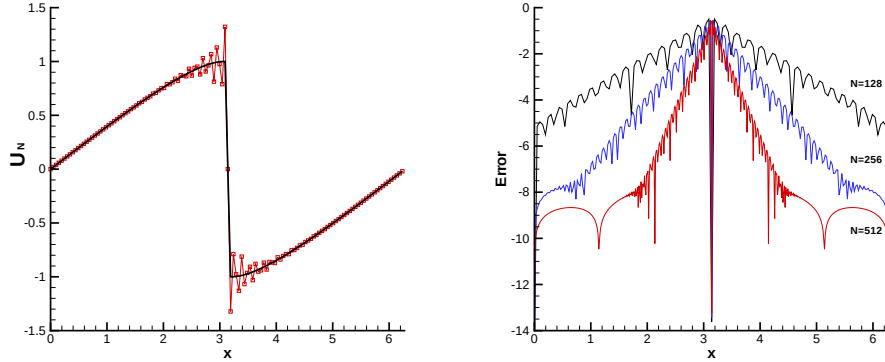
Fig. 3. (Left) Exact and Fourier spectral solution of the Burgers equation with a 16-th order Exponential filter and N = 128 collocation points. (Right) Convergence of the solution with N = 128, 256, 512 . The error is in the log10 scale.
