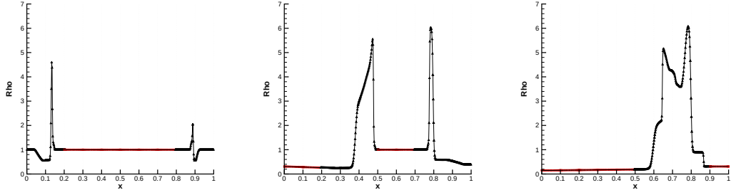
(a) t = 0.014 \mathbf{w^2 s^6 w^2} (b) t = 0.16 \mathbf{s^2 w^3 s^2 w^3} (c) t = 0.38 \mathbf{s^5 w^4 s^1}
