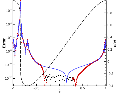
Fig. 5. (Dashed line) Inviscid Burgers Equation solution; (Continuous line) Error of the fifth-order classical WENO with 400 points; (Symbols) Error of the Hybrid method.
