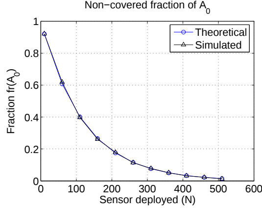
Fig. 2. Fraction fr(\mathcal{A}_0) of \mathcal{A}_0 , that remains non-covered as a function of the number of sensors N that are deployed to monitor the field of interest.
