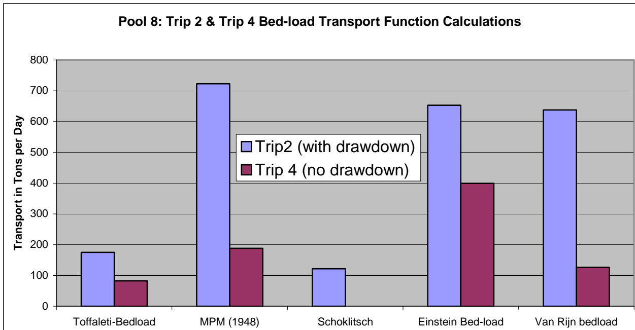
Figure 10. Results of transport function calculations for bed-load transport through study reach
