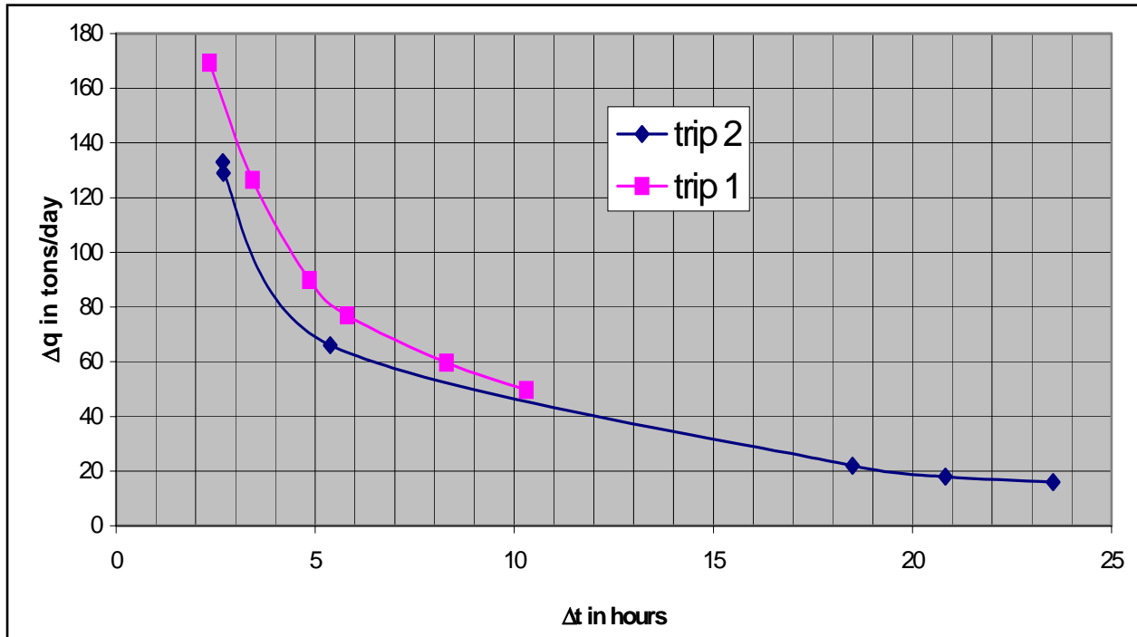
Figure 3. \Delta q versus \Delta t as computed using ISSDOT for stated conditions (Tons/day vs. time span between measurement of two sections. Values are average of 30 rows at each \Delta t )
