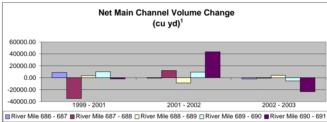
Figure 7. Main channel volume change by year for study area locations
