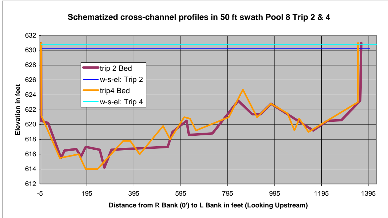
Figure 9. Comparison of channel cross sections in study area for trips 2 and 4
