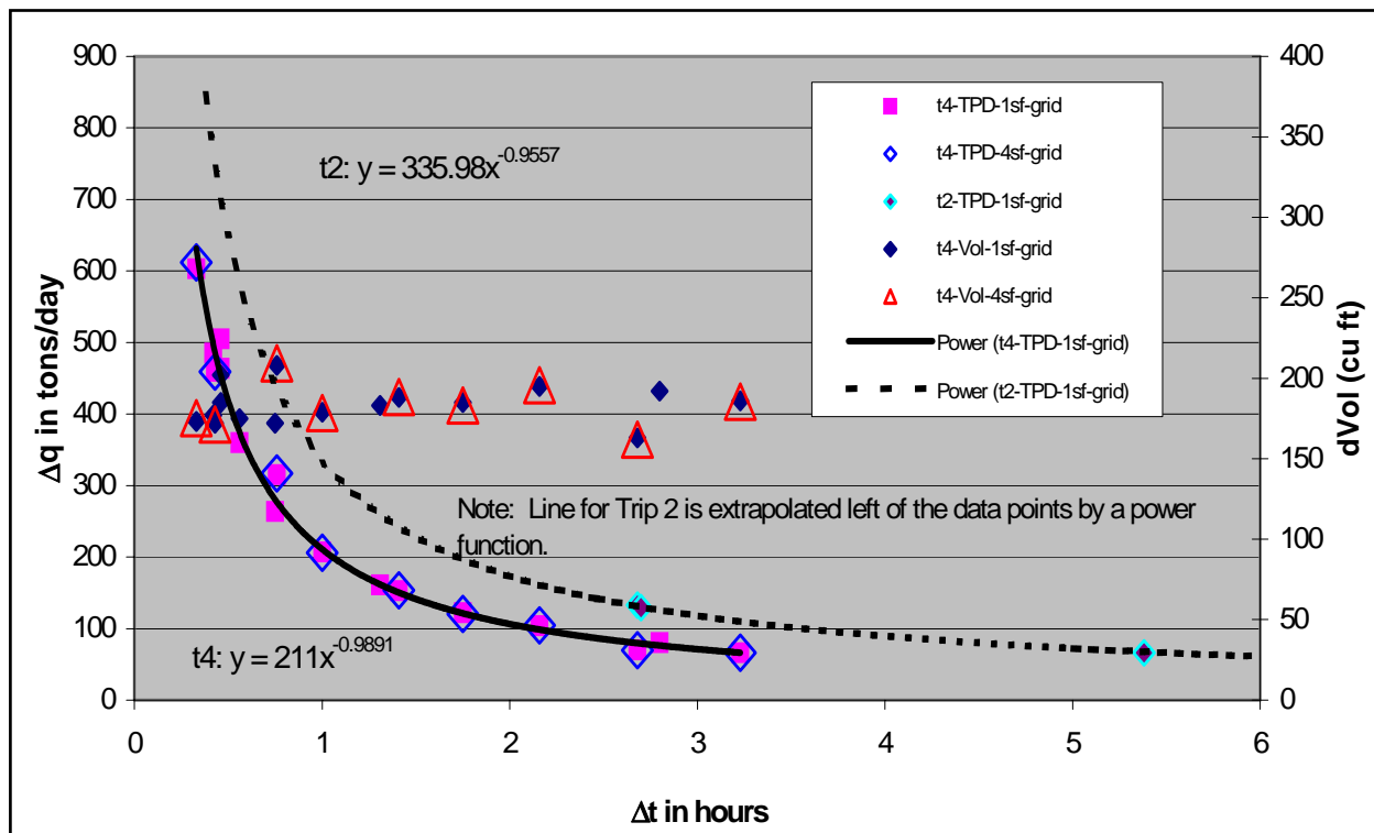
Figure 4. \Delta q versus \Delta t computed using ISSDOT for stated conditions change in volume used to compute \Delta q for each \Delta t is also shown (Tons/day vs. time span between measurement of two sections. Average of 30 rows at each \Delta t . Data from trip 4 and 2)
