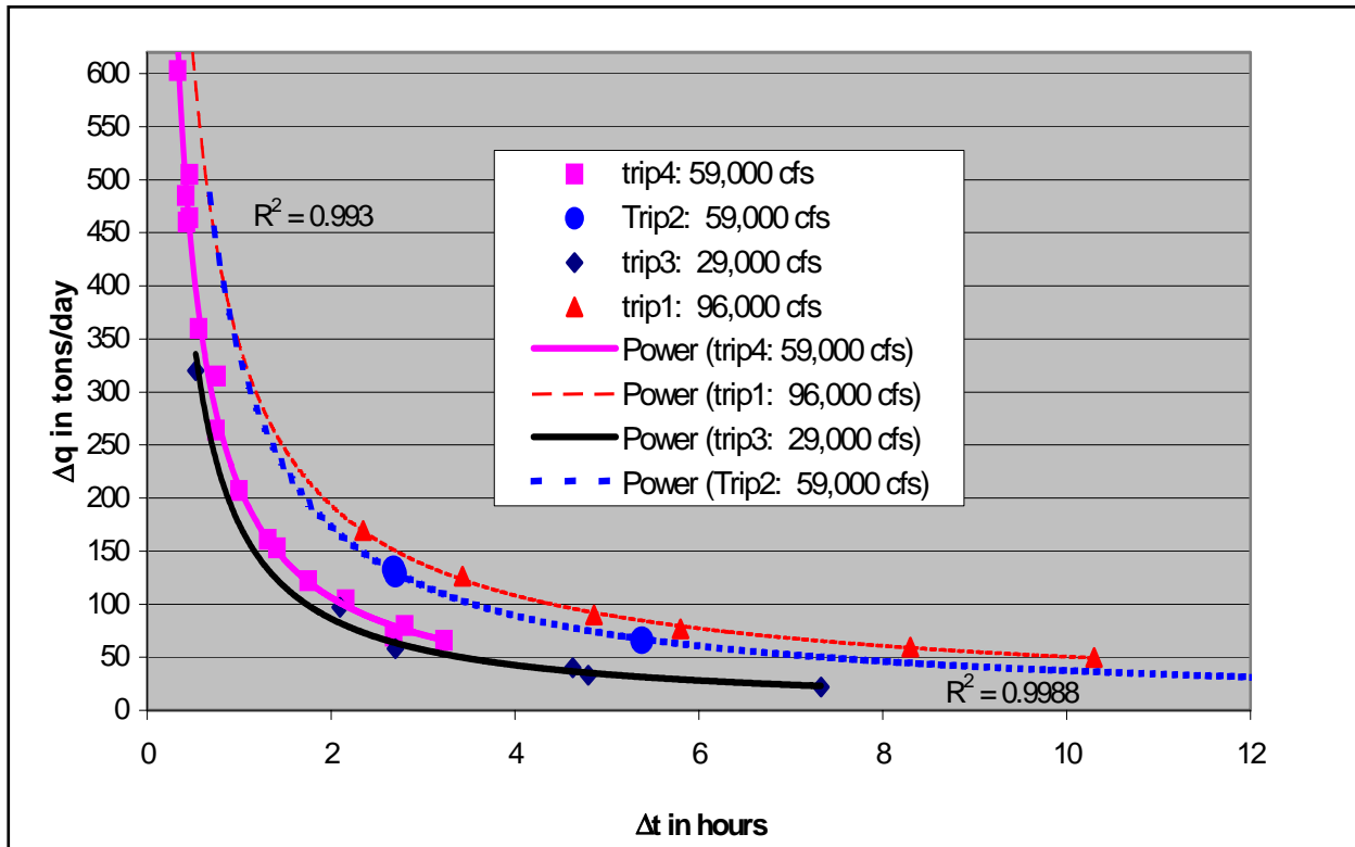
Figure 5. \Delta q versus \Delta t computed using ISSDOT for stated conditions (Tons/day vs. time span between measurement of two sections. Average of 30 rows at each \Delta t . Data from trip 1, 2, 3 and 4)
