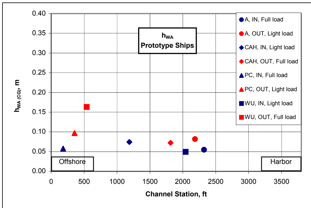
Figure 11. Maximum h_{WA(CG)} for the four prototype ships
