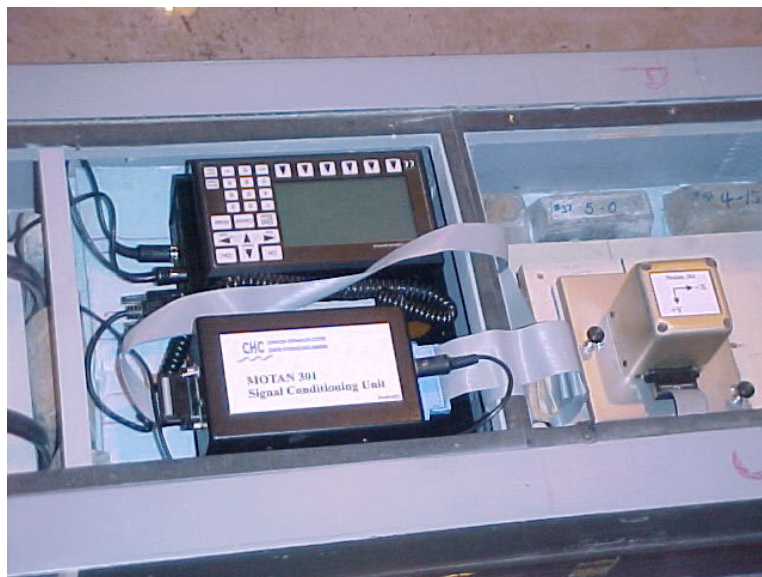
Figure 7. MOTAN motion analysis system installed in the model ship
