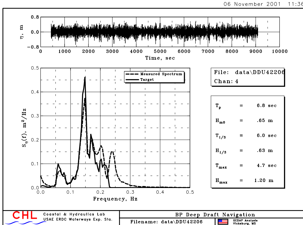
Figure 9. Target and laboratory wave case DDU422 for T_p = 6.7 sec and H_{m0} = 0.58 m
