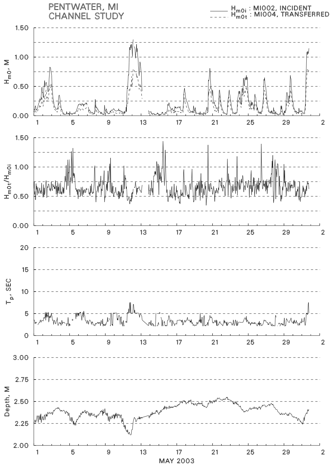
Figure 3: MI002 & MI004 H_{m0} comparison, transfer rates, and MI002 T_p and depth for May 2003.
