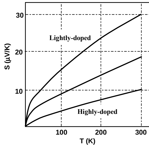
Fig. 3 Typical Seebeck coefficient of conjugated polymers as a function of temperature [4,7,13].
