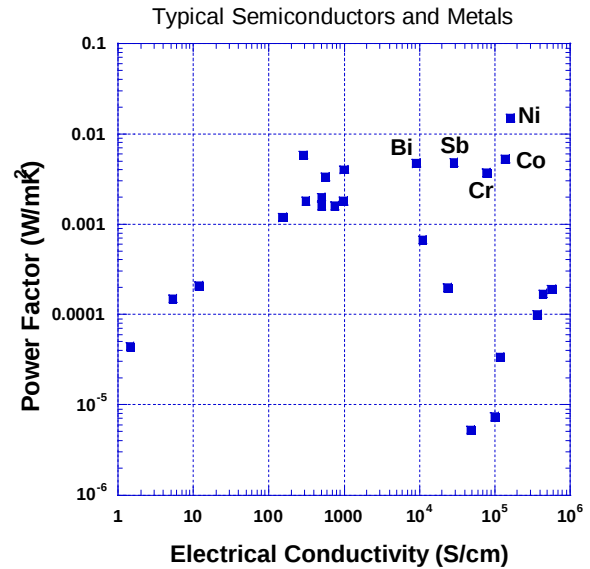
Fig. 4 Power factor as a function of electrical conductivity for various semiconductors and metals (see Table 1).
