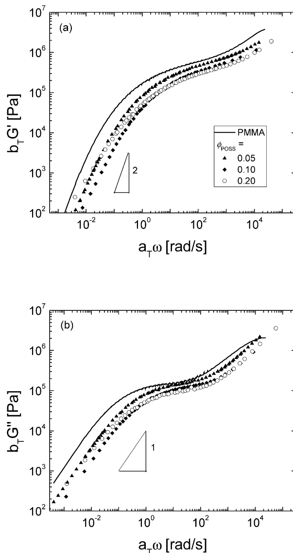
Fig. 6. Master curves at T_0 = 170^\circ\text{C} for (a) the storage modulus G' and (b) the loss modulus G'' of hydrogenated acrylic-POSS-PMMA blends.
