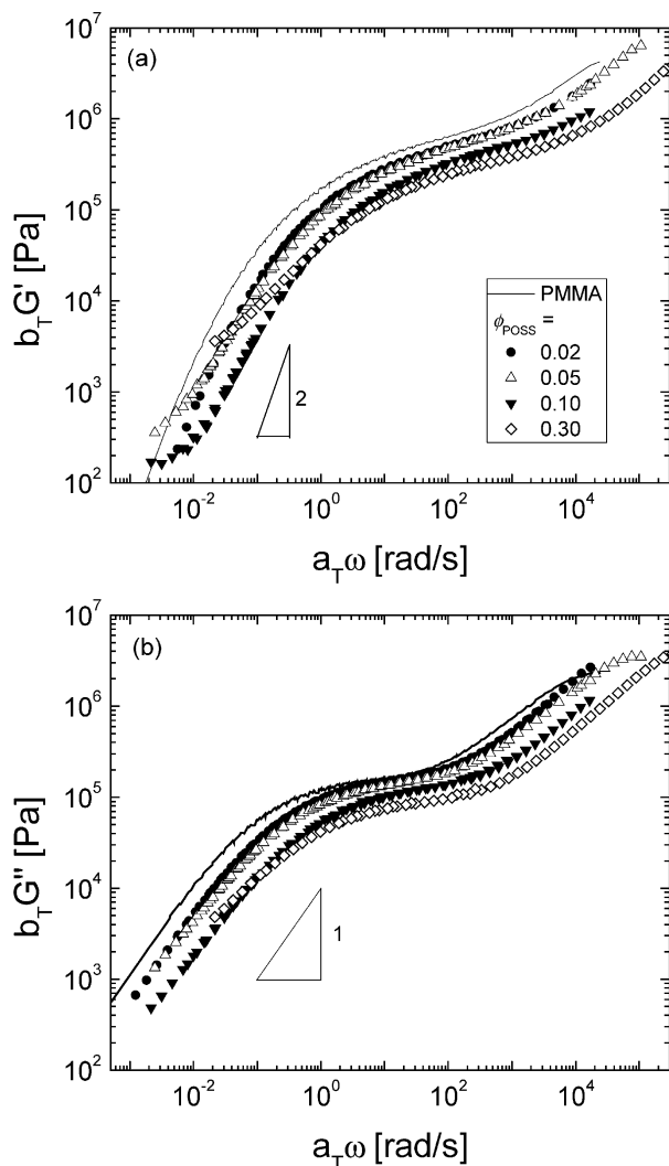
Fig. 5. Master curves at T_0 = 170^\circ\text{C} for (a) the storage modulus G' and (b) the loss modulus G'' of unmodified acrylic-POSS-PMMA blends.
