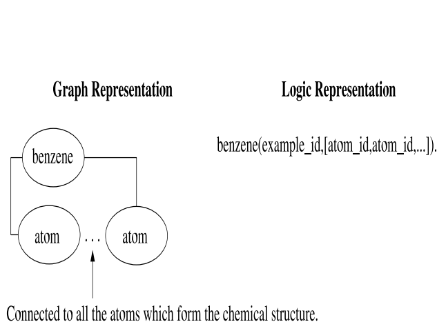
Figure 8: Representation of the Mutagenesis dataset while comparing the ability to utilize background knowledge indicating generic chemical concepts.
