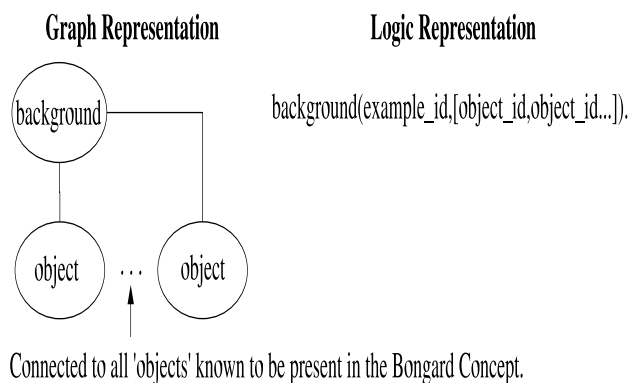
Figure 9: Representation for introducing background knowledge in Bongard Problems.
