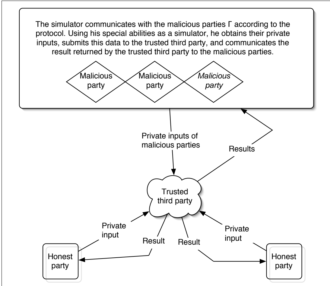
Figure 3.1: Basic outline of a standard simulation proof.
