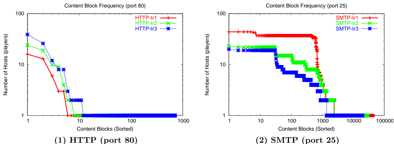
Figure 5.8: Number of hosts (players) that have generated each content block (item) from observed suspicious flows.
