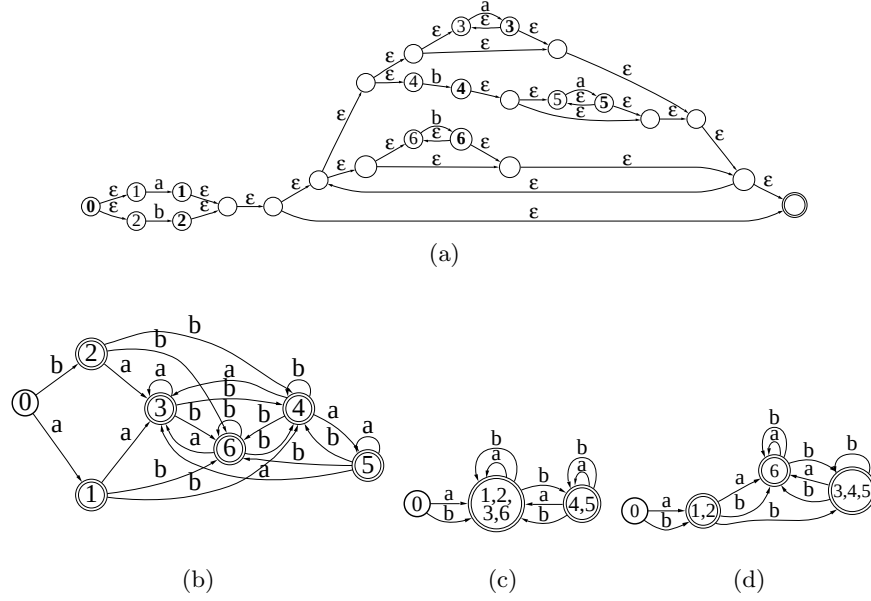
Fig. 1. (a) The Thompson automaton, (b) Glushkov automaton, (c) Follow automaton, and (d) Antimirov automaton representing the regular expression \alpha = (a+b)(a^* + ba^* + b^*)^* . This regular expression is the running example from [13].
