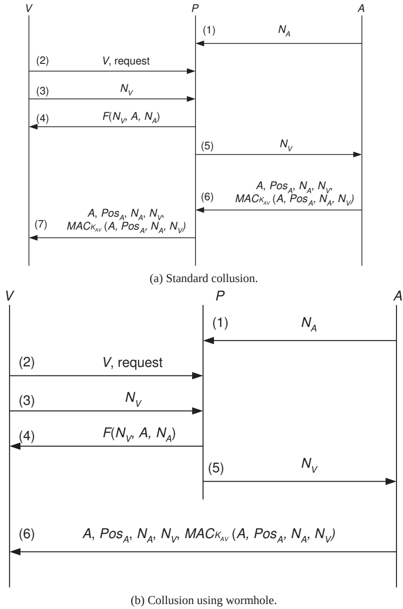
Fig. 2. Protocols under Collusion of nodes A and P
