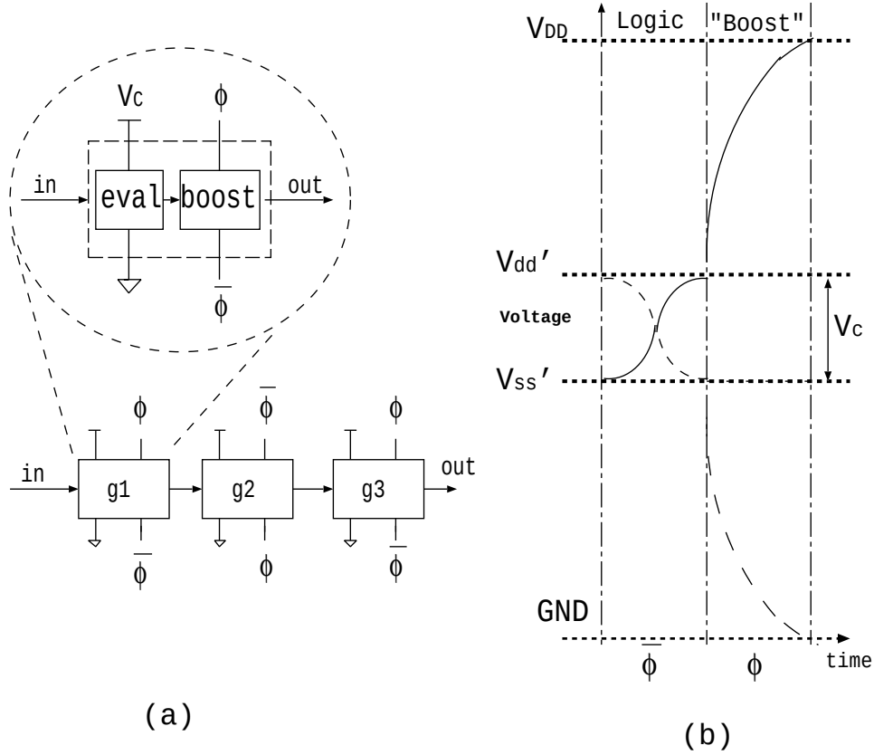
Figure 1: Boost Logic (a) Cascade and (b) Operation
