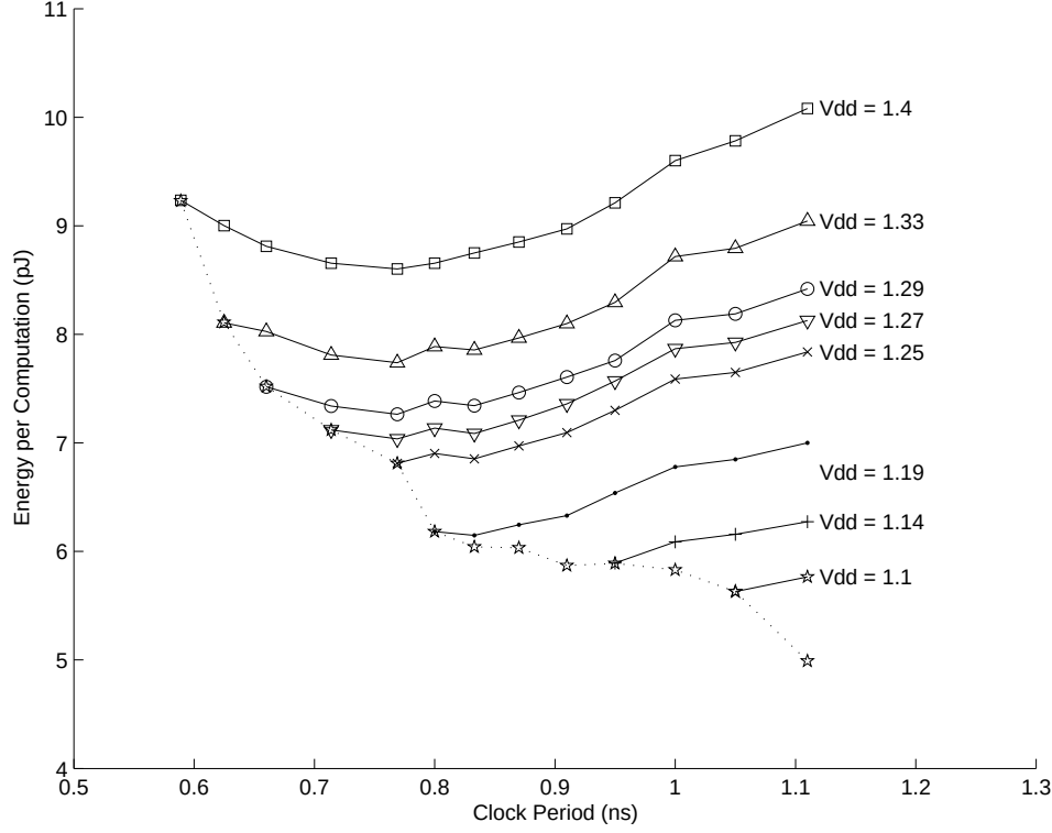
Figure 9: Energy-Delay variation in 8-bit array multiplier
