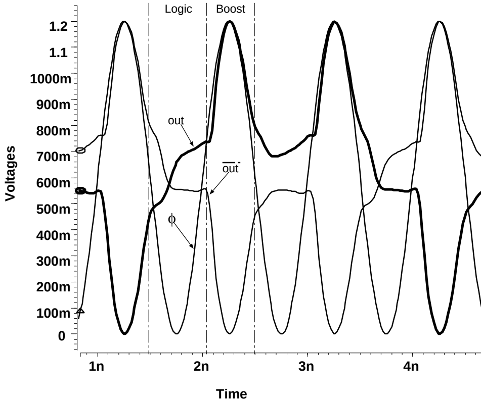
Figure 3: SPICE waveforms of a Boost Logic inverter
