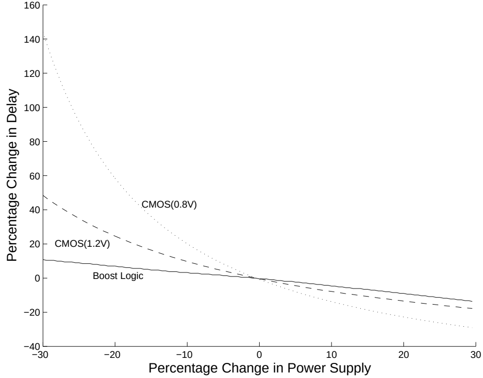
Figure 6: Effect of power supply variation from nominal values on delay in Boost and CMOS NAND gates
