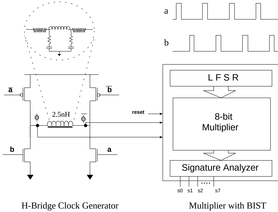
Figure 8: Overall simulation setup
