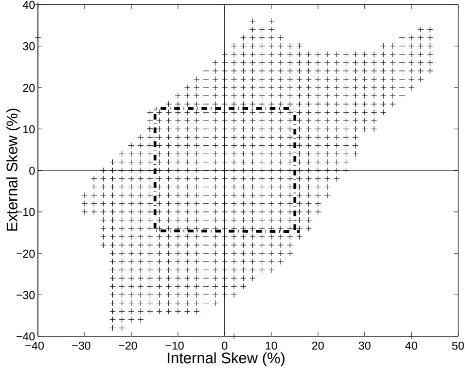
Figure 5: Schmoor plot for functional correctness over a range of internal and external skew values
