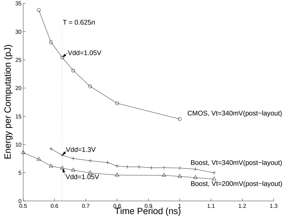
Figure 11: Energy consumption vs frequency for 8-bit multipliers
