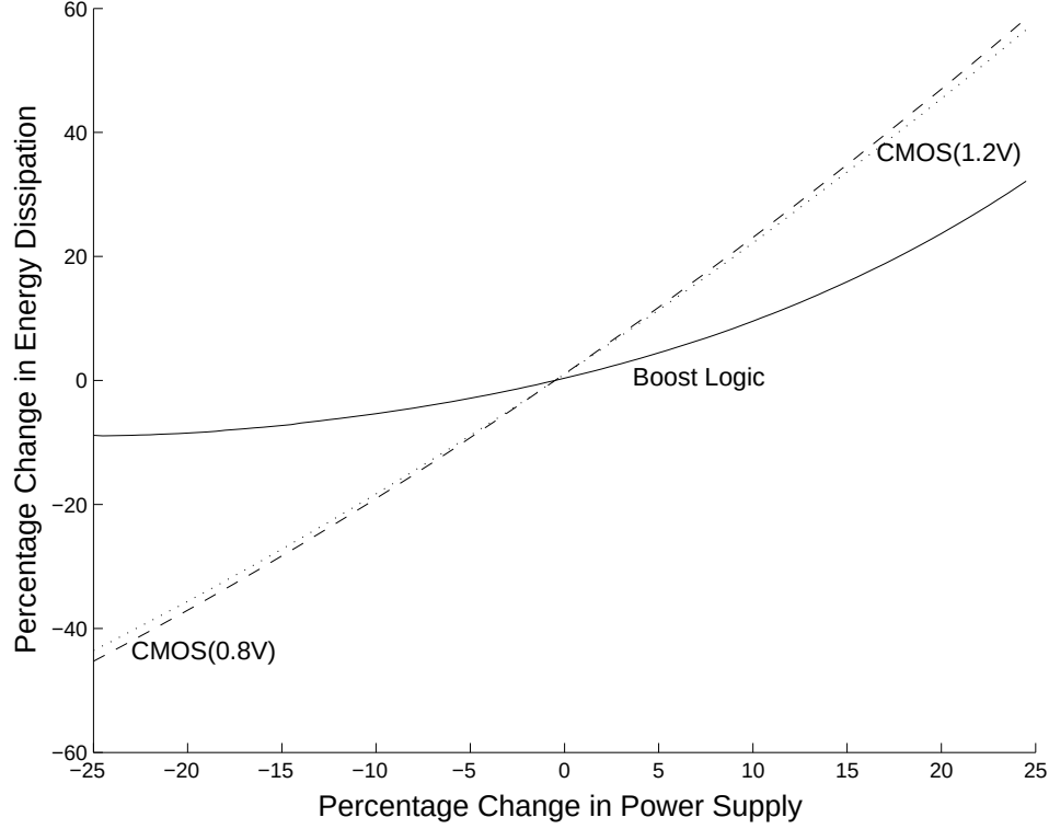
Figure 7: Effect of power supply variation from nominal values on energy dissipation in Boost and CMOS NAND gates
