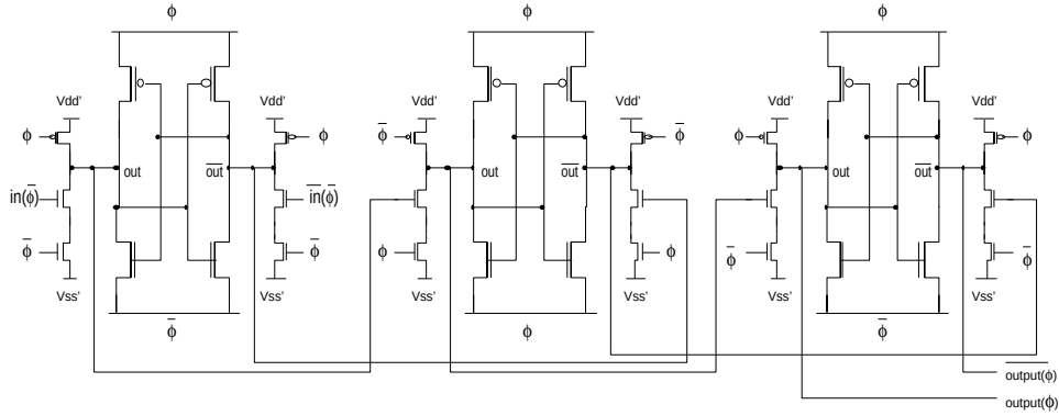
Figure 4: Cascade of Boost Logic inverters
