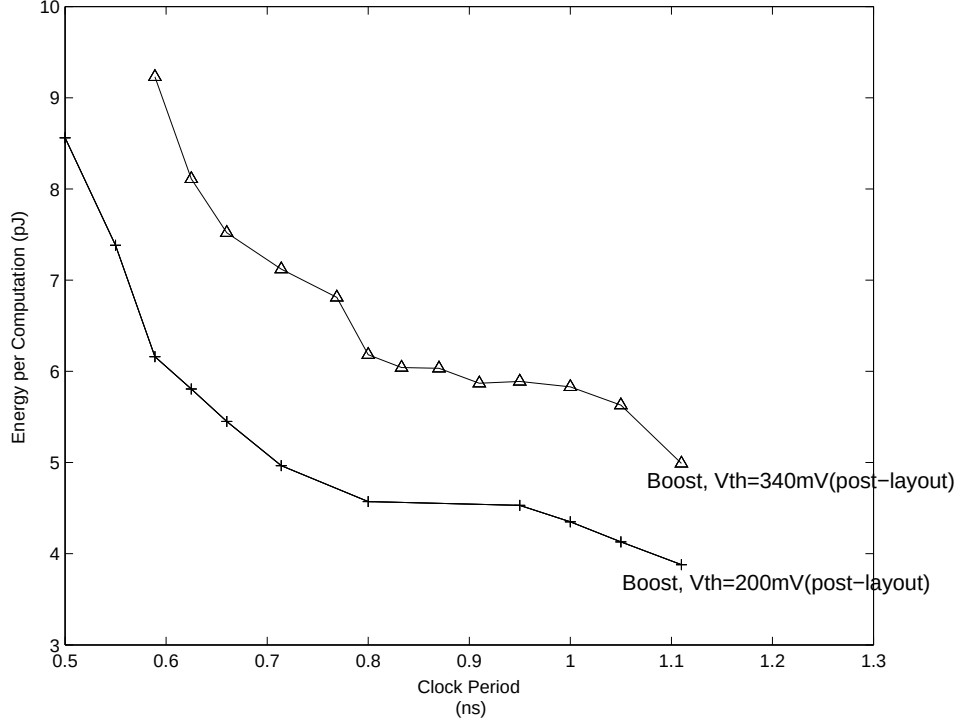
Figure 10: Energy delay curves for nominal V_{th} and low V_{th} 8-bit Boost multipliers
