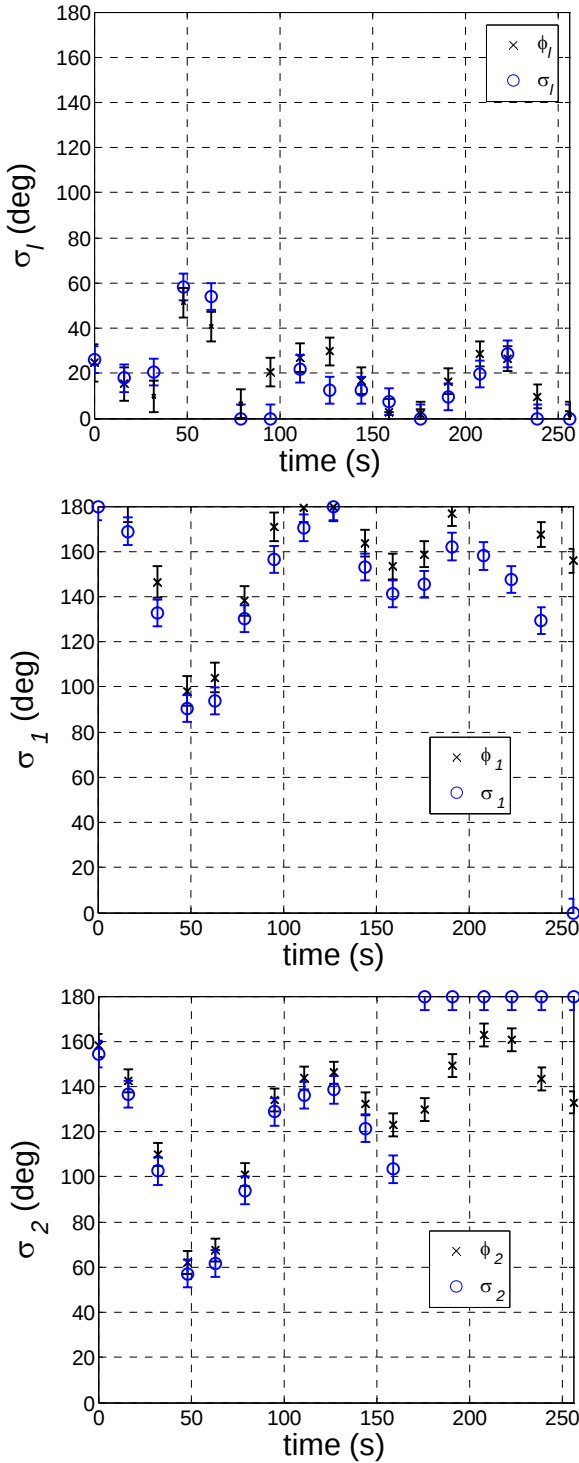
Fig. 3 Bearing angles to leader and fixed transponders as determined by follower two-hydrophone sensor and GPS data.
