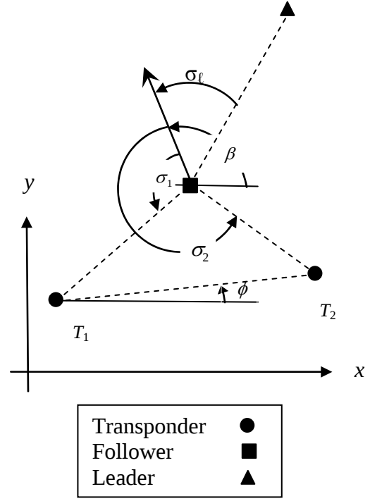
Fig. 1 Vehicle and transponder geometry.
