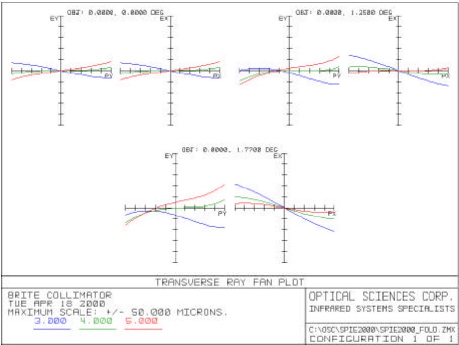
Figure 6. Ray Fans
