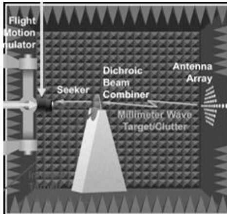
Figure 1. Chamber Schematic
