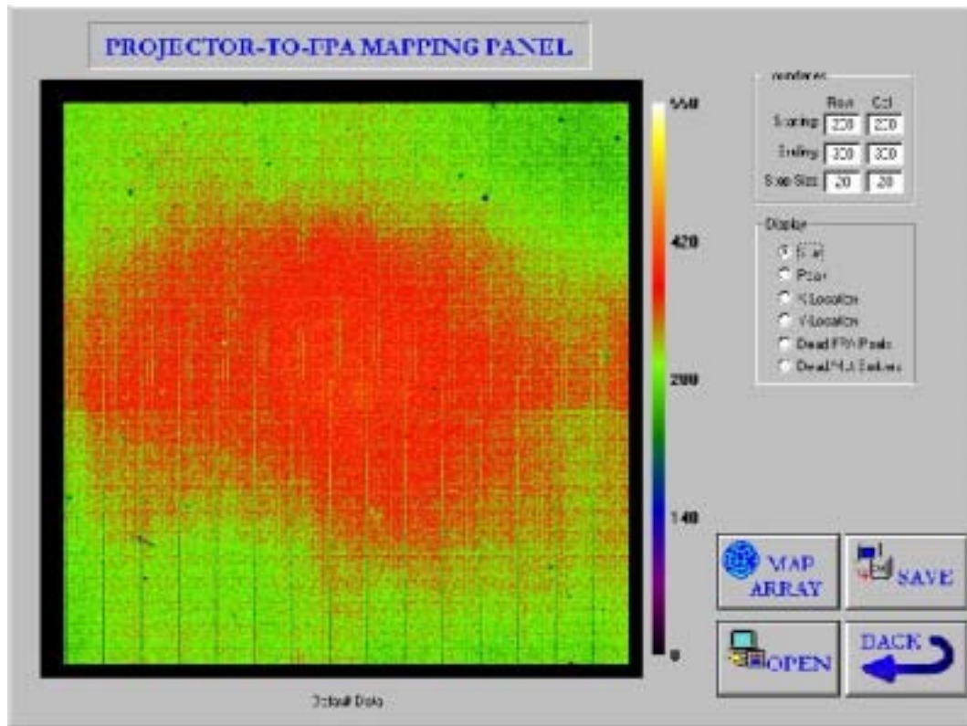
Figure 9: AMCOM IRSP SCS Emitter Array Mapping Panel
