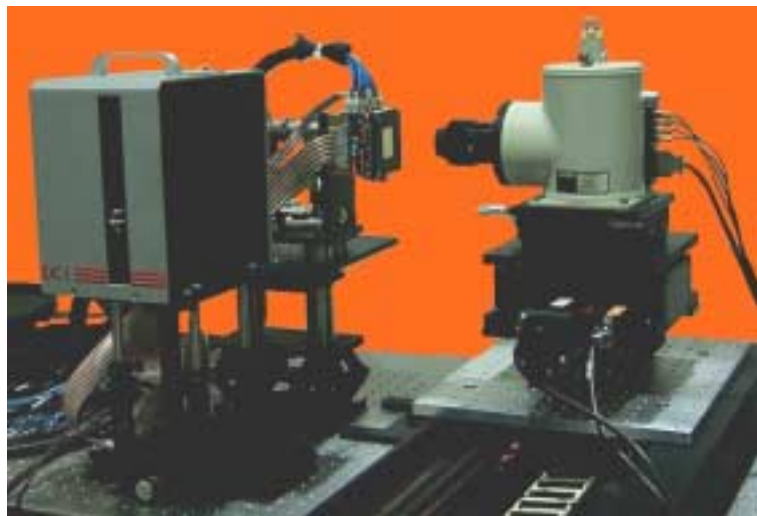
Figure 12 – Emitter array non-uniformity correction and characterization station
