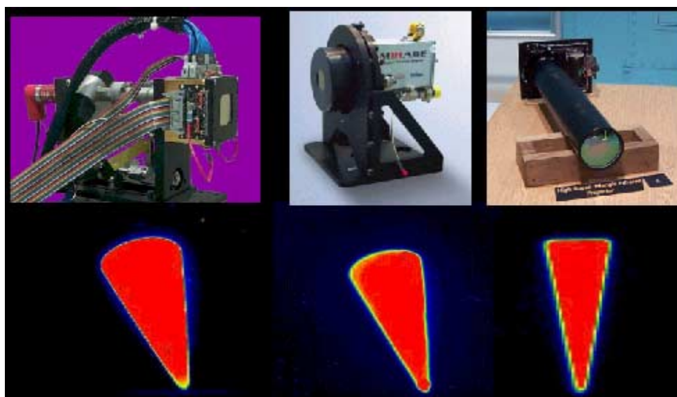
Figure 2: Dynamic IRSP Technologies and Example 'RV' Imagery
