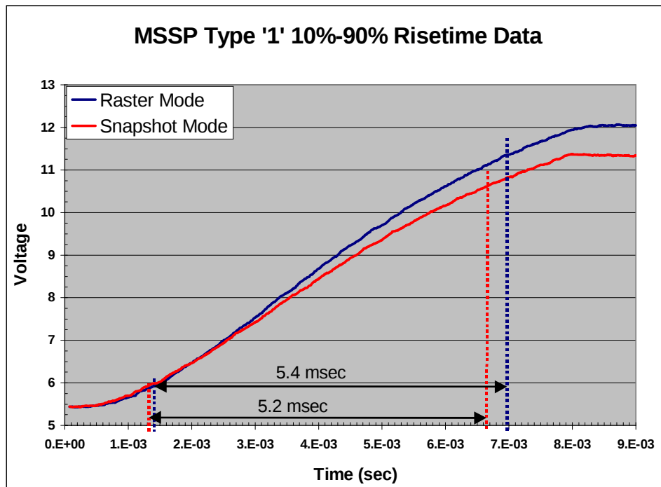
Figure 3: MSSP Raster and Snapshot Risetime Values
