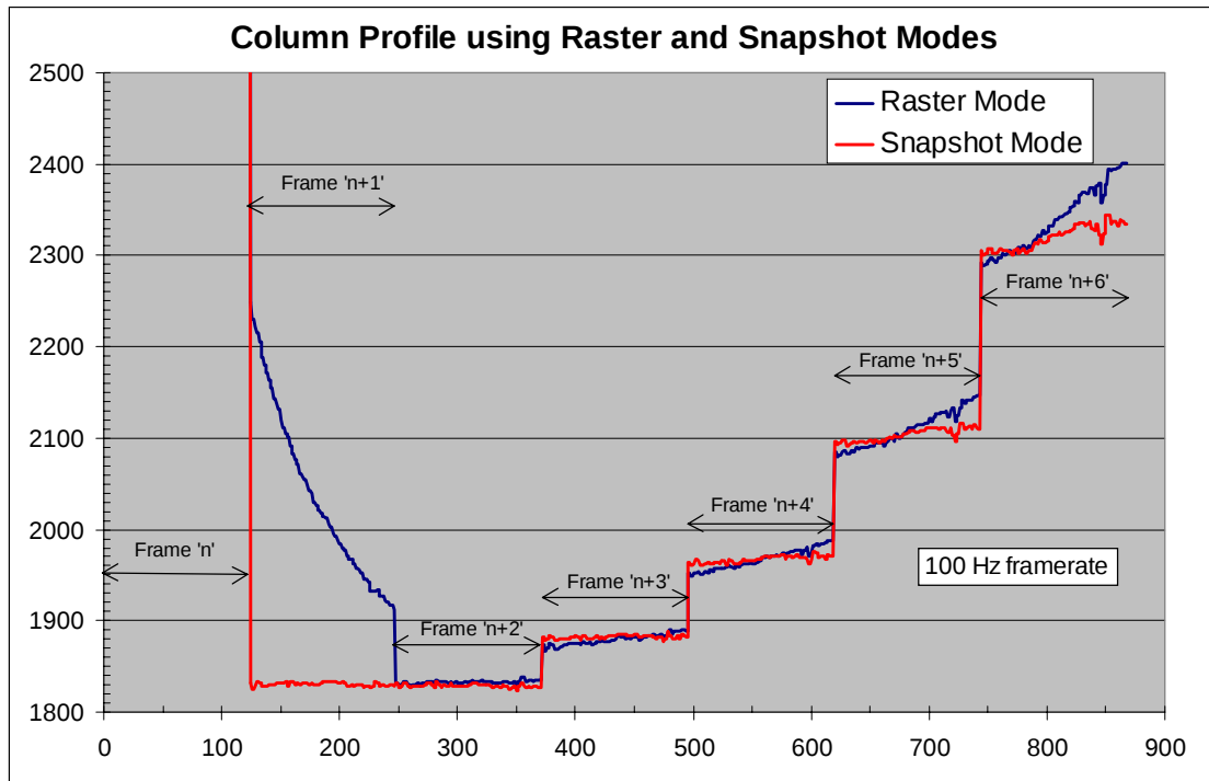
Figure 4: Comparison of MSSP Raster and Snapshot Update Mechanisms
