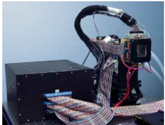
Figure 5: AMCOM IRSP Analog Electronics
