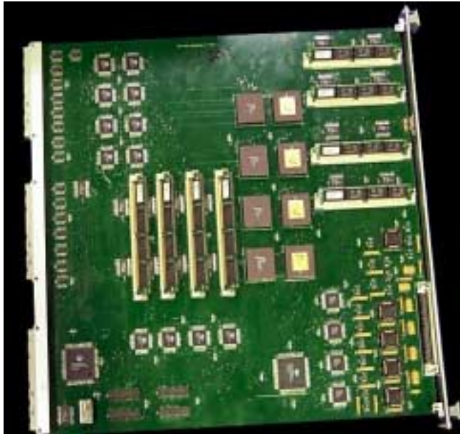
Figure 6: AMCOM IRSP Digital Board
