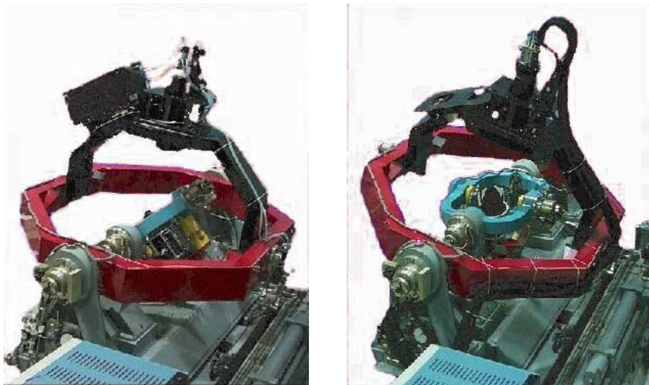
Figure 1: Integration of Honeywell Emitter IRSP (left) and MIRAGE IRSP (right) into TMD HWIL test entry.
