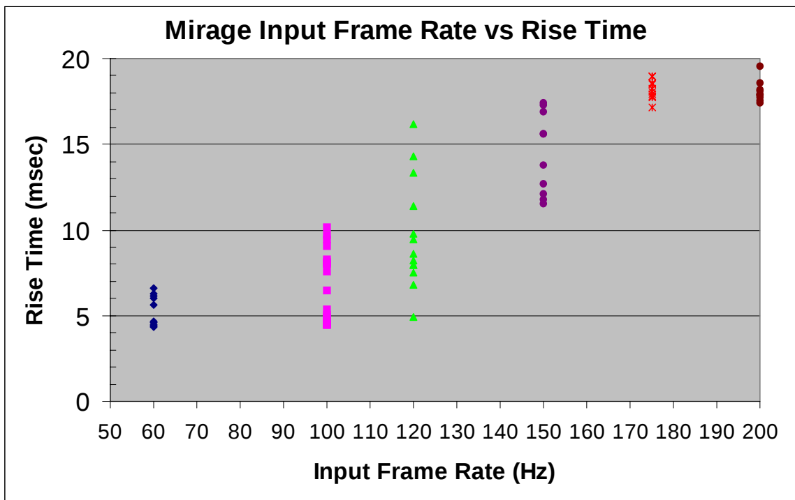
Figure 14: MIRAGE Overdrive Risettime Measurements
