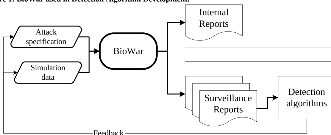
Figure 1: BioWar used in Detection Algorithm Development.
