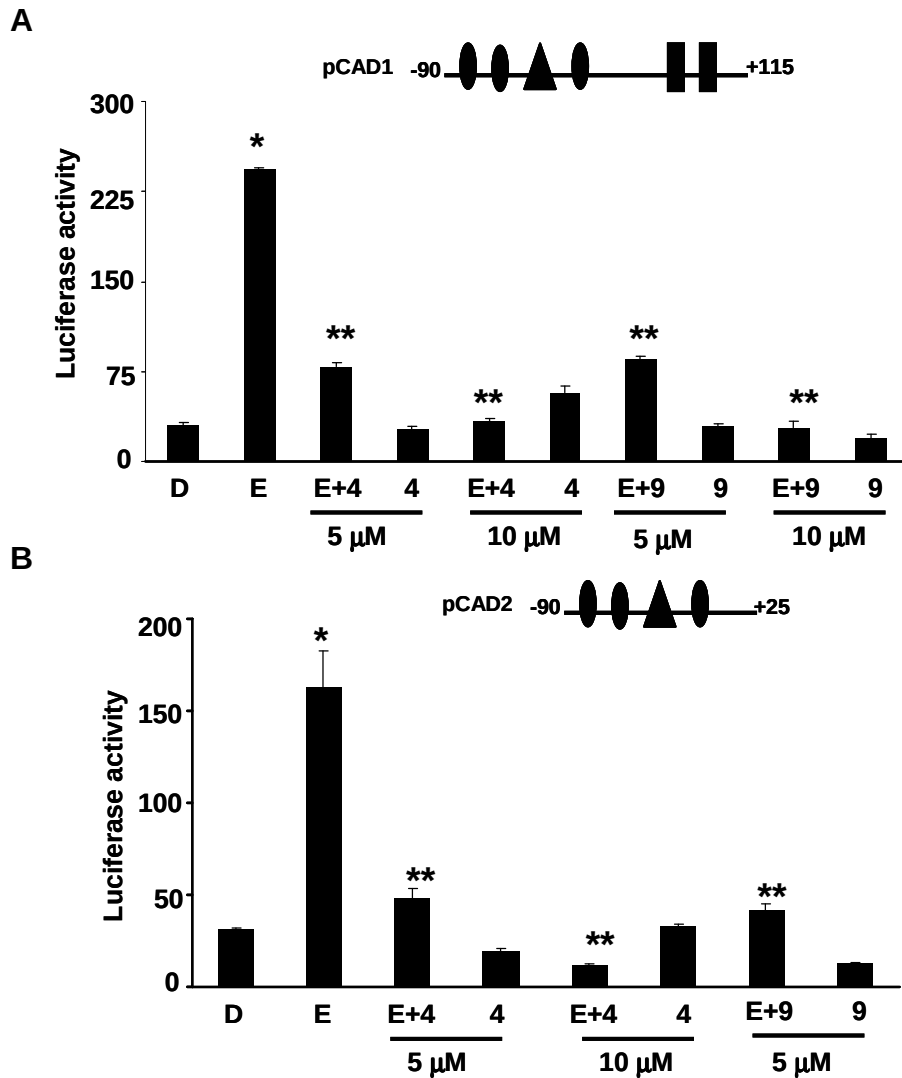
Figure 16. Inhibition of estrogen-induced transactivation in cells transfected with pCAD constructs and treated with DIM-C-pPhBu (# 4) and DIM-C-pPhC6H5 (# 9) in MCF-7 cells. MCF-7 cells were transfected with pCAD constructs, pCAD1 [A] or pCAD2 [B] treated with DMSO (D), 10 nM E2, # 4 or # 9 alone, or in combination with E2 [E+ #4 or E+ # 9] and luciferase activities were determined. Results are expressed as means \pm SD for at least three replicate determinations for each treatment group and significant ( p < 0.05 ) induction by E2 (*) or inhibition by E2 plus # 4 (**) or E2 plus # 9 (**) are indicated.
