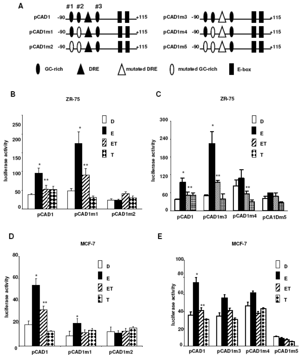
Figure 5. Inhibitory AhR-ER \alpha crosstalk in cells treated with wild-type or mutant CAD constructs. [A] Summary of CAD constructs and their cis elements. Transfection of wild-type and mutant CAD constructs in ZR-75 [B and C] and MCF-7 [D and E] cells. Cells were transfected with the constructs, treated with DMSO, 10 nM E2, 10 nM TCDD, or E2 plus TCDD, and luciferase activity determined was determined. Results are expressed as means \pm SE for three replicate determinations for each treatment group and significant ( p < 0.05 ) induction by E2 (*) or inhibition by E2 plus TCDD (**) are indicated.
