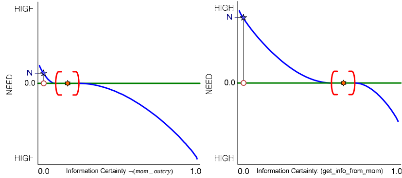
Fig. 4. Information Certainties and NEEDs of \neg(\text{mom\_outcry}) and (\text{get\_info\_from\_mom})
