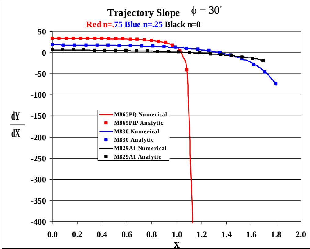
Figure 2. Comparison of analytic and numeric trajectory slopes.
