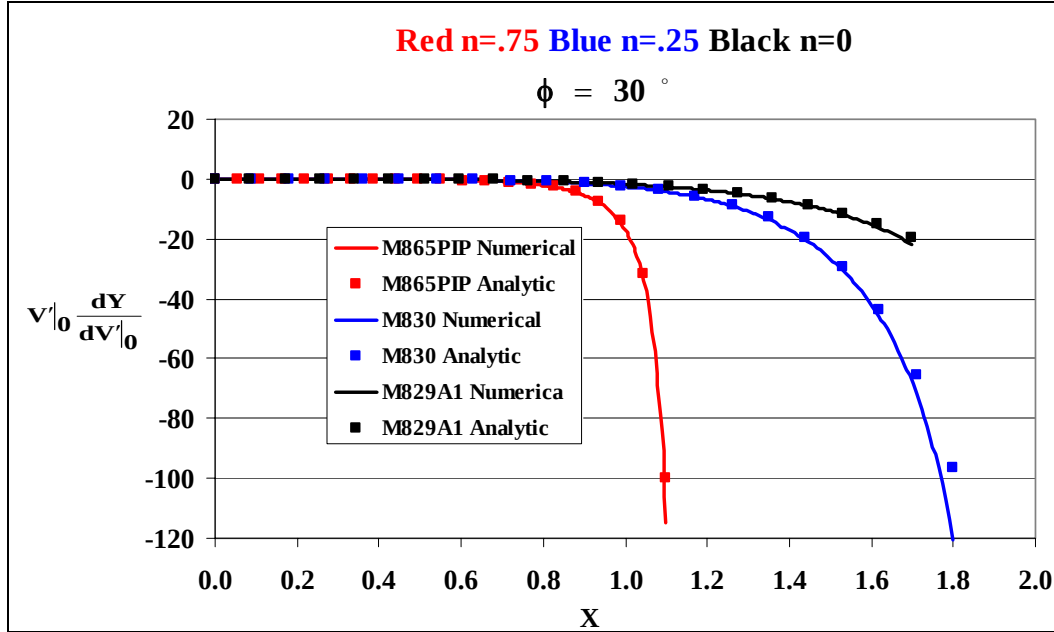
Figure 8. Comparison of scaled numerical and analytic dy/dV'_0 .
