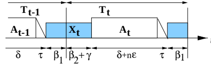
Figure 3.12: Prototypical STR timeline.
