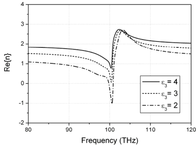
Fig. 9. Calculated real part of the refractive index of nano coated-spheres dispersed nematic liquid crystal film as the director axis orientation is realigned [electrically or optically].
