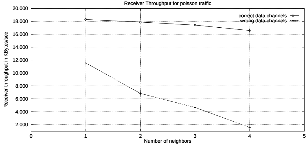
Figure 6.9: Receiver throughput at node 2 with varying number of 1-hop neighbors, Average Interarrival time = 0.05 seconds
