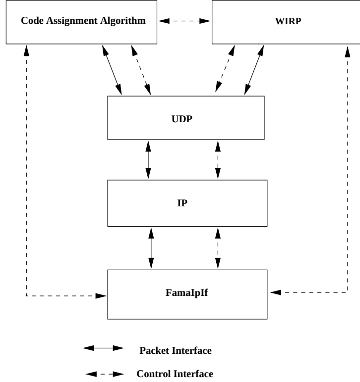
Figure 6.1: Stack used for implementation
