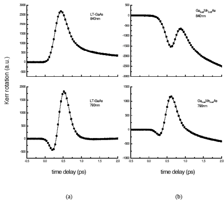
Fig.2 Short-term dynamics of Kerr rotation in LT-GaAs (a) and Ga 0.95 Mn 0.05 As (b) at different wavelengths.
