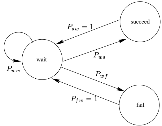
Fig. 1. Markov chain model for a node
