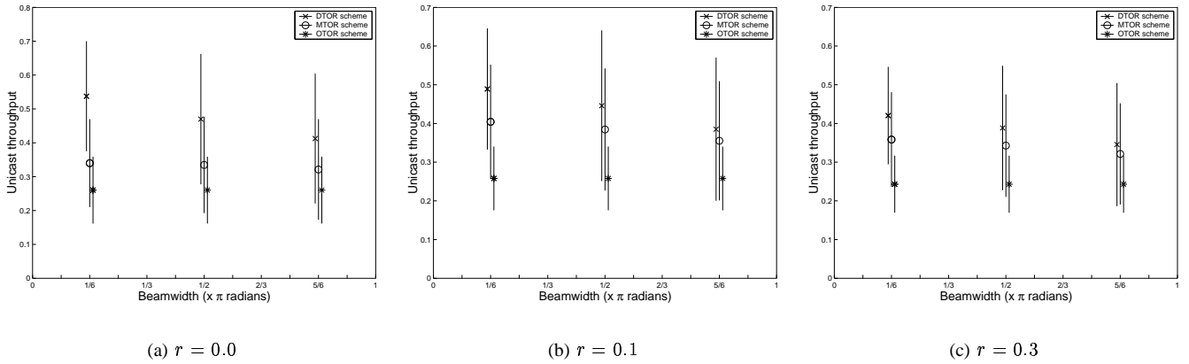
Fig. 11. Unicast throughput with broadcast traffic ( N = 5 )
