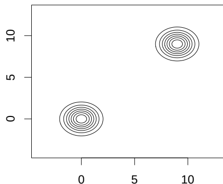
Figure 1: Density contours for a mixture of 2 unit-variance bivariate normals
