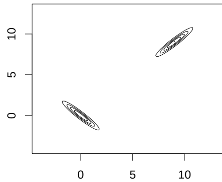
(f) TwoNarrow
