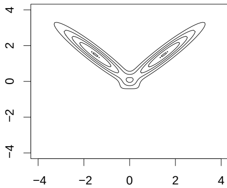
(e) Banana
