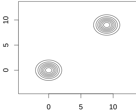
(c) TwoMode
