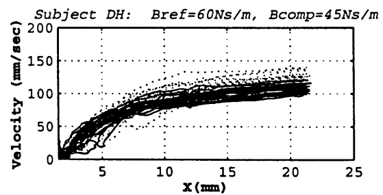
Figure B.16 Velocity Data for Subject DH with Reference Viscosity = 60Ns/m. Velocity data plotted versus time and squeezing distance for all stimulus pairs. Solid lines are for trials where the reference was presented and dotted lines represent trials where the comparison was presented.
