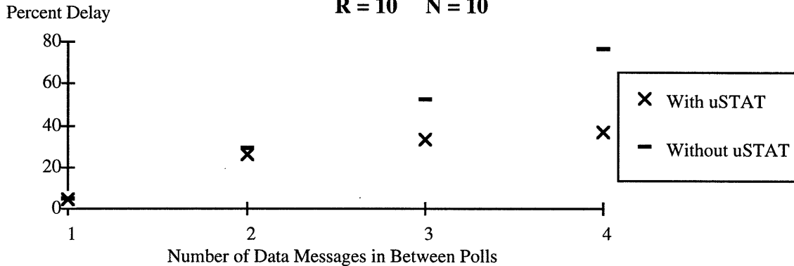
Graph 3 Percent Expected Relative Excess Delay vs. Interval Between Polls R = 10 \quad N = 10
