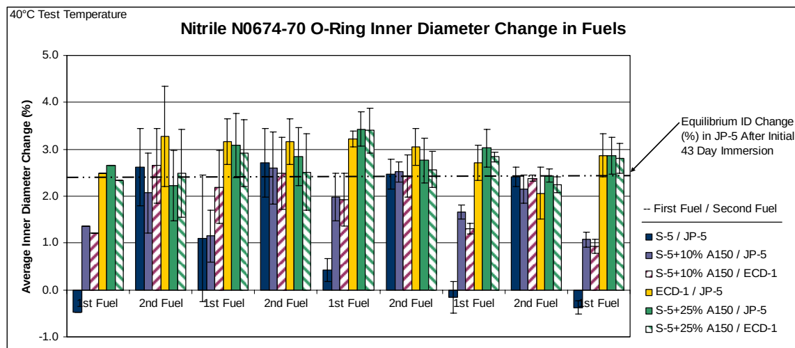
Figure E-5. Inner Diameter Change (%) for Nitrile N0674-70 O-Ring Switch-Loaded between Fuels
