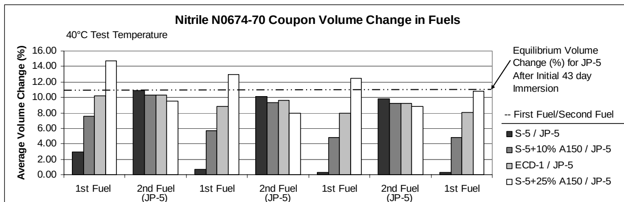
Figure 4. Volume Change (%) for Nitrile N0674-70 Coupon Switch-Loaded between Fuels
