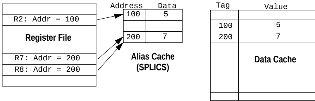
Figure 8. The SRF Alias Cache.
