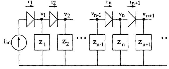
Figure 3-3: Diode ladder network.
