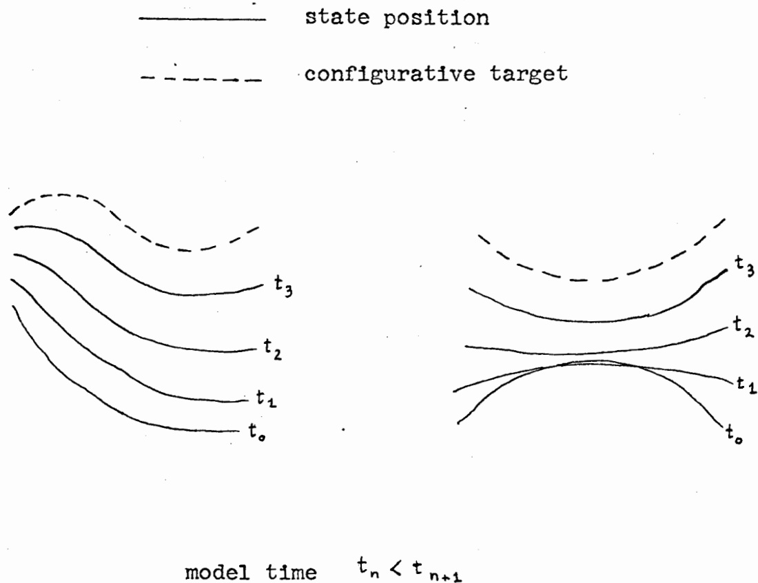
Fig. 3.1 Hypothetical state trajectories as effected by the position and shape seeking mechanism. Shape seeking functions independently of the location of the state position with respect to the configurative target. Note in the right hand example that a part of the structure temporarily regressed in the position sense since a large shape change was needed. The shape influence was effectively "stronger" than the position influence.
