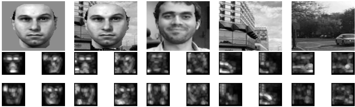
Figure 2-2: Typical stimuli and associated responses of the C1 complex cells (4 orientations). Top: Sample synthetic face , cluttered face, real face, non-faces. Bottom: The corresponding C1 activations to those images. Each of the four subfigures in the C1 activation figures maps to the four bar orientations (clockwise from top left: 0, 45, 135, 90 degrees). For simplicity, only the response at one scale is displayed. Note that an individual C1 cell is not particularly selective either to face or to non-face stimuli.
