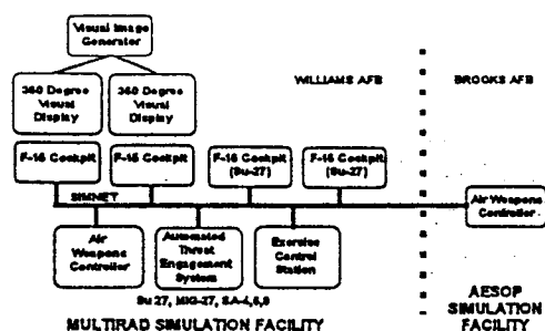
Figure 3. Armstrong Laboratory Simulation Facility
