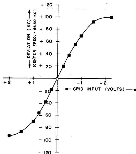
Fig. 10 - Frequency shift (fm) modulator
