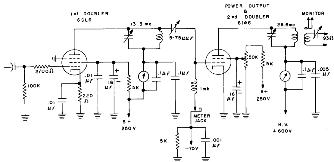
Fig. 8 - Doubler circuit
