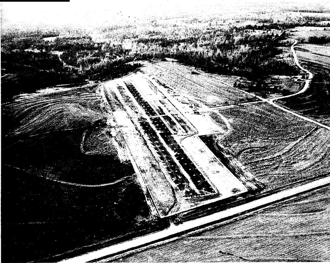
Fig. 11 - Jordan Lake transmitting antenna field
