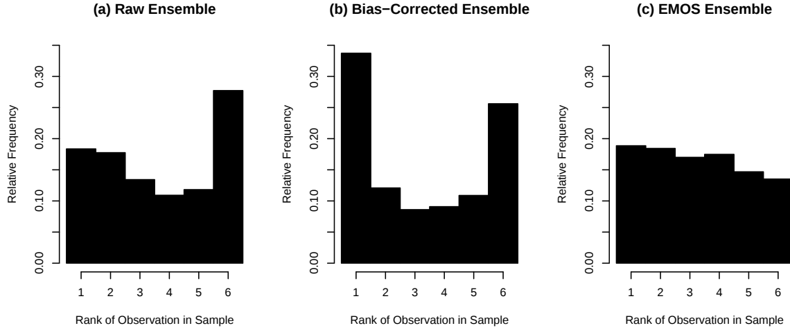
Figure 5: Verification rank histograms for ensemble forecasts of sea level pressure over the Pacific Northwest: (a) Raw ensemble. (b) Bias-corrected ensemble. (c) EMOS ensemble.
