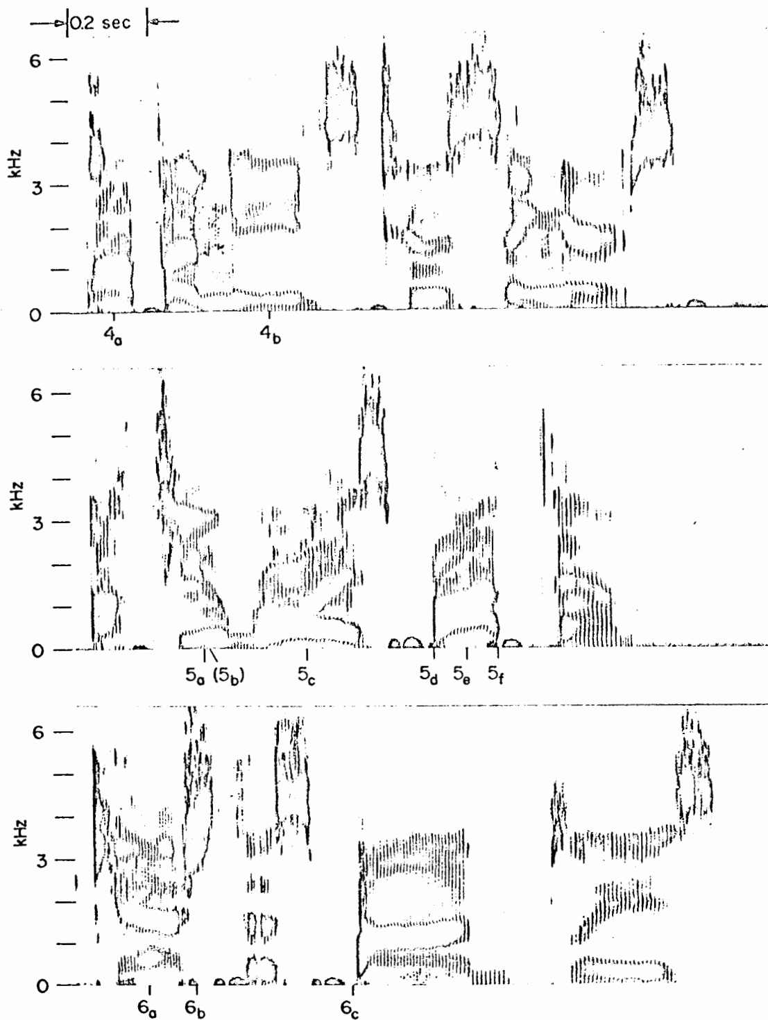
Figure 5. Spectrograms of sentences 4, 5, 6. Top: Papa needs two singers. Middle: A few boys bought them. Bottom: Cash this bond please.
